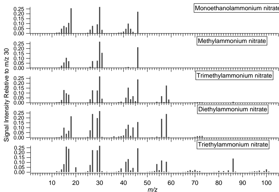
Fig. 2. Mass spectra for the nitrate salts of the amines studied. On the \sim 550^\circ\text{C} surface of the vaporizer, all nitrate salts decompose into nitric acid and the parent amine. Signals at m/z 30 and 46 are generated from the nitrate fragments \text{NO}^+ and \text{NO}_2^+ and are common to all spectra. Signal at m/z 30 is a combination of signal from \text{NO}^+ and from amine fragments resulting from rearrangements after electron impact ionization. For all spectra, molecular ions have significantly less signal intensity than the fragments resulting from the cleavage of the chemical group alpha to the nitrogen (alpha cleavage). For the ethyl amines, loss of methyl groups alpha to the nitrogen give fragments at [\text{M}-15]^+ while for the methyl amines, loss of hydrogen atoms alpha to the nitrogen give fragments at [\text{M}-1]^+ .
