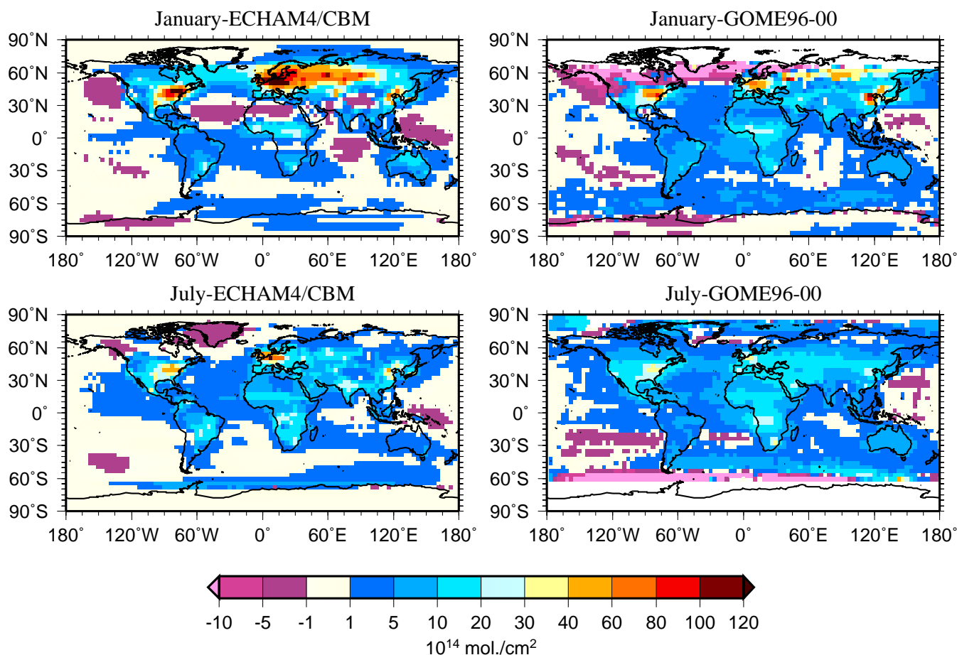
Fig. 2. Tropospheric NO 2 columns [ 10^{14} mol. \text{cm}^{-2} ] derived from GOME satellite data (right) (Richter and Burrows, 2002) and ECHAM4/CBM model simulations (left) for January (top) and July (bottom).
