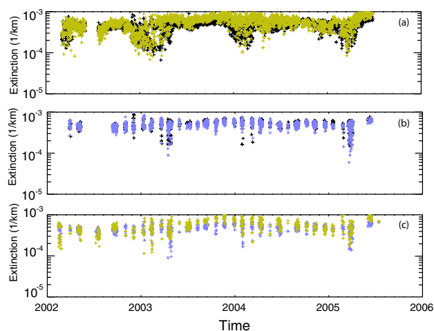
Fig. 4. This figure shows 18 km, aerosol extinction coefficient near 450-nm as measured by SAGE III, SAGE II, and POAM II using the match requirements described in the text. Frame (a) shows POAM III (gold) matched with SAGE III (black); frame (b) shows SAGE III (black) matched with SAGE II (blue); and frame (c) shows SAGE II (blue) matched with POAM III (gold).
