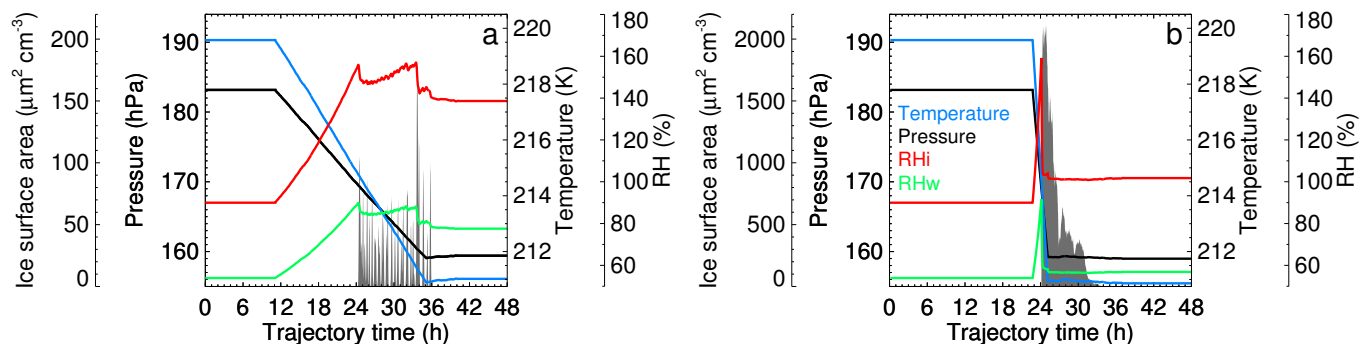
Fig. 1. Ambient conditions and cirrus ice surface area concentrations (gray areas) along the slow (a) and fast (b) updraft trajectories, generated with a 1D cirrus model (Jensen and Pfister, 2004). RHi and RHw denote the relative humidity over a flat ice and a flat water surface, respectively.
