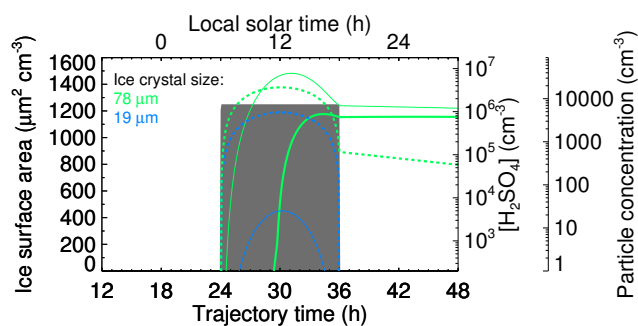
Fig. 5. Aerosol formation in two idealized cirrus clouds with an ice surface area concentration of 1250 \mu\text{m}^2 \text{cm}^{-3} (gray area), at constant conditions of 170 hPa, 210 K, and 150 % relative humidity over ice. The first cloud consists of 19 \mu\text{m} , the second of 78 \mu\text{m} ice crystals. The day length is 12 h, the noon OH volume mixing ratio 0.3 ppt, and the \text{SO}_2 volume mixing ratio 1 ppb in both cases. Preexisting aerosol surface area concentration has been set to zero. Broken lines represent the \text{H}_2\text{SO}_4 concentration, thin solid lines the concentration of supercritical aerosol particles, thick solid lines the concentration of aerosol particles with diameters >3 nm. Nucleation is negligible in the presence of the smaller, but vigorous in the presence of the larger ice crystals. In the latter case, >3 nm diameter aerosol particles are produced in vast numbers.
