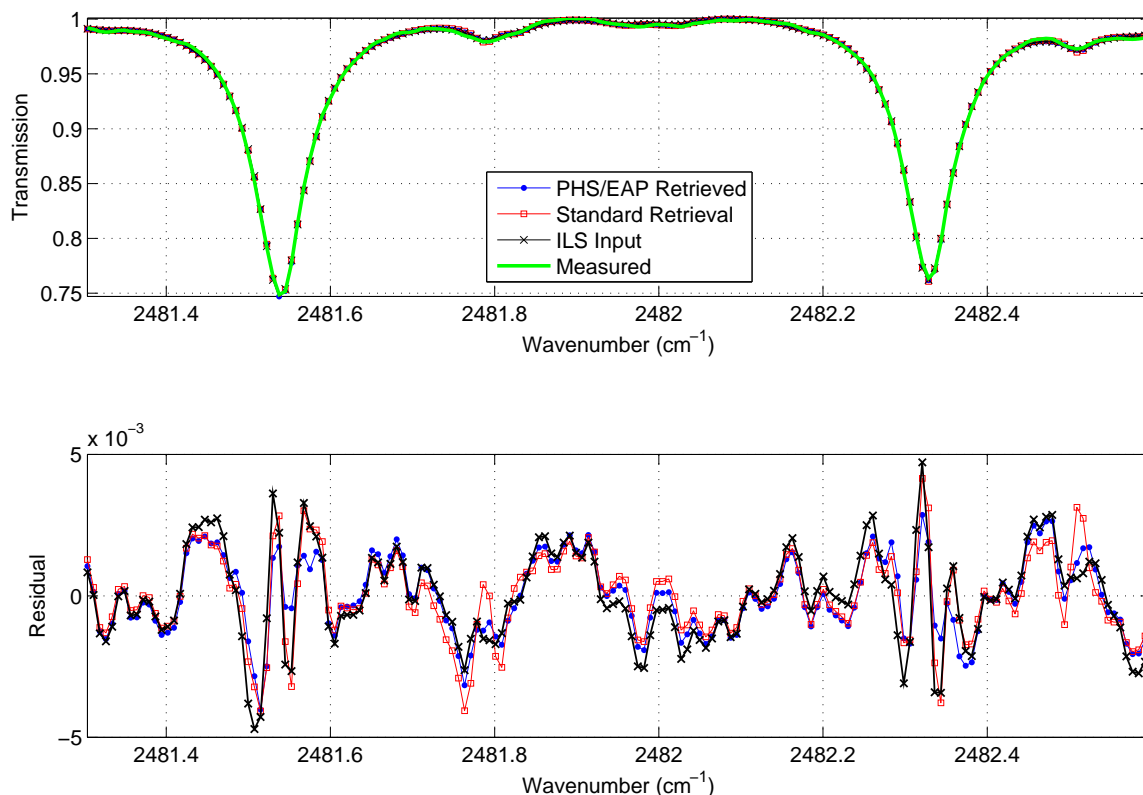
Fig. 11. N 2 O spectral fits for the U of T FTS (upper panel), and the corresponding residuals (lower panel).
