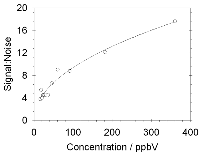
Fig. 8. Signal: noise ratio versus concentration for the OVOC 2-hexanone. Data fit with a power law, equation: S/N = 1.0017 \times \text{Concentration}^{0.4866} .
