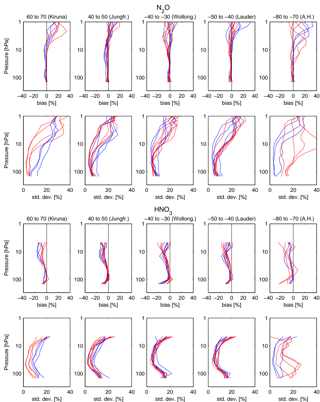
Fig. 5. Monthly zonal mean bias and standard deviation (std. dev.) between BASCOE and MIPAS profiles of N 2 O (top) and HNO 3 (bottom), in 10° latitude bands around ground-based stations (A.H.: Arrival Heights). In blue: December to May; in red: June to November. For polar regions, monthly statistics are shown only for months where FTIR provides observations. Latitude are specified in °N.
