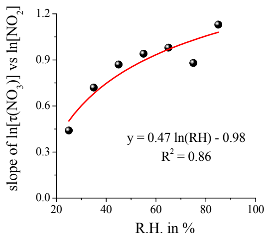
Fig. 9. Correlation of the slope of the regression of \ln[\tau(\text{NO}_3)] versus the \ln[\text{NO}_2] (data from Fig. 8) as a function of R.H.
