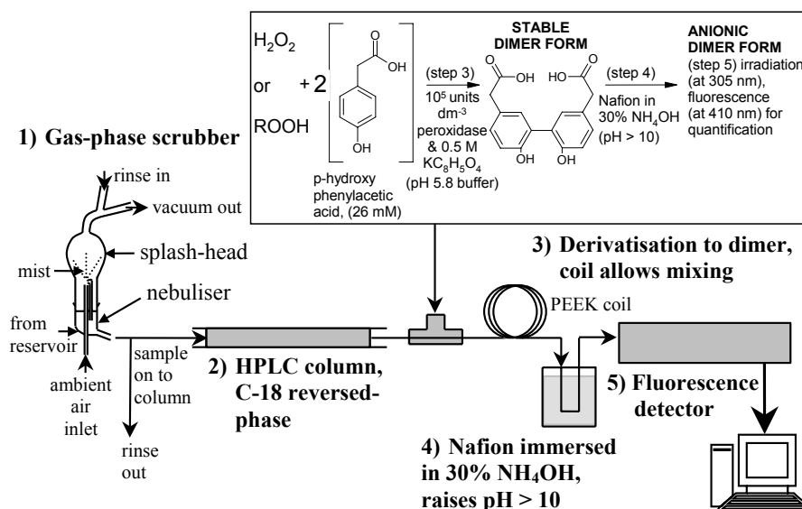
Fig. 3. Schematic diagram of gas-phase sampling and analysis of hydroperoxides using a nebulising reflux concentrator, HPLC and post-column derivatisation.
