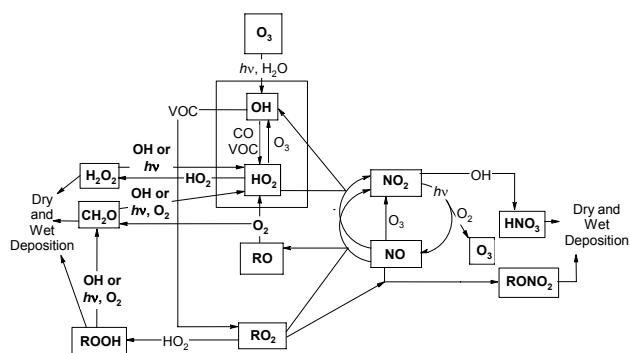
Fig. 1. Tropospheric gas-phase reactions linked to hydroperoxides.
