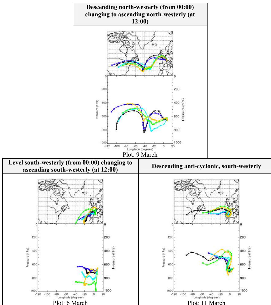
Fig. 2. Typical 5-day back-trajectories of air-masses sampled at JFJ (provided by the BADC Trajectory Server). Arrival dates of trajectories are shown. Trajectory release times are 00:00 (black), 06:00 (dark blue), 12:00 (light blue), 18:00 (green) and 24:00 (orange) in GMT. Crosses are every 6 h along trajectory.
