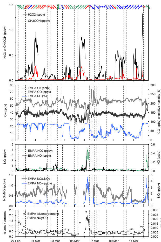
Fig. 4. Time series of \text{H}_2\text{O}_2 , \text{CH}_3\text{OOH} , \text{O}_3 , \text{CO} , relative humidity (RH), \text{NO}_2 , \text{NO} , \text{NO}_y , \text{NO}_x to \text{NO}_y , toluene to benzene and \text{NO}_y to \text{CO} ratios. Arrows in top panel and dashed vertical lines indicate changes in the prevailing wind direction deduced from the last day of 5-day back-trajectories (see Sect. 3.2 for further details). Descending air from >3.6 km (blue arrows), ascending air from <2 km (red arrows) and level (green arrows) indicates air that had remained at constant altitude for the last 5 days. Local \text{NO} and toluene contamination has been removed. Tick marks on time axis refer to noon (GMT).
