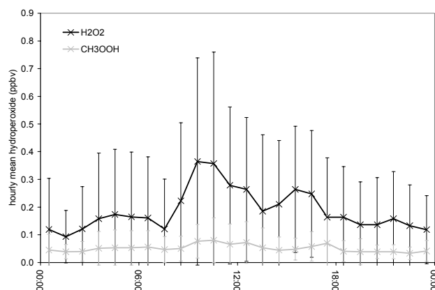
Fig. 5. Hourly averaged diurnal cycles for \text{H}_2\text{O}_2 (black crosses/line) and \text{CH}_3\text{OOH} (grey crosses/line) where error bars show 1 standard deviation.
