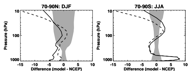
Fig. 4. Zonally averaged temperature difference in K between the models and NCEP in the high latitude winter hemisphere averaged between 1979–1999. Models with a high top are averaged together and displayed with a solid line and models with a low top are averaged together and displayed with a dashed line. The differences are computed for DJF (left) and JJA (right). The gray shading indicates the 1 sigma standard deviation in the NCEP reanalysis.
