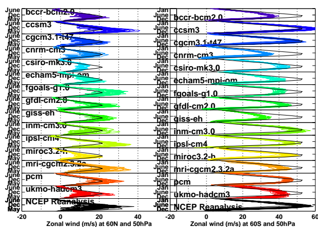
Fig. 5. Time series of zonally averaged zonal wind at 60° N (left) and 60° S (right) at 50 hPa between the year 1979–1999 for a subset of the submitted IPCC models and the NCEP reanalysis. Each of the 20 years of data is plotted on top of each other and compared to the 20 year mean NCEP reanalysis given in the black bold line.
