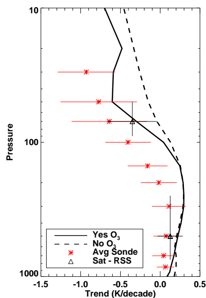
Fig. 9. As in Fig. 8 except for the tropical trend ( 30^{\circ} N– 30^{\circ} S) between 1979–1999 trend. Satellite observations are given by the triangle symbol, where the thin vertical line represents the 2-sigma uncertainty and the thin vertical line represents the approximate vertical range of the observations.
