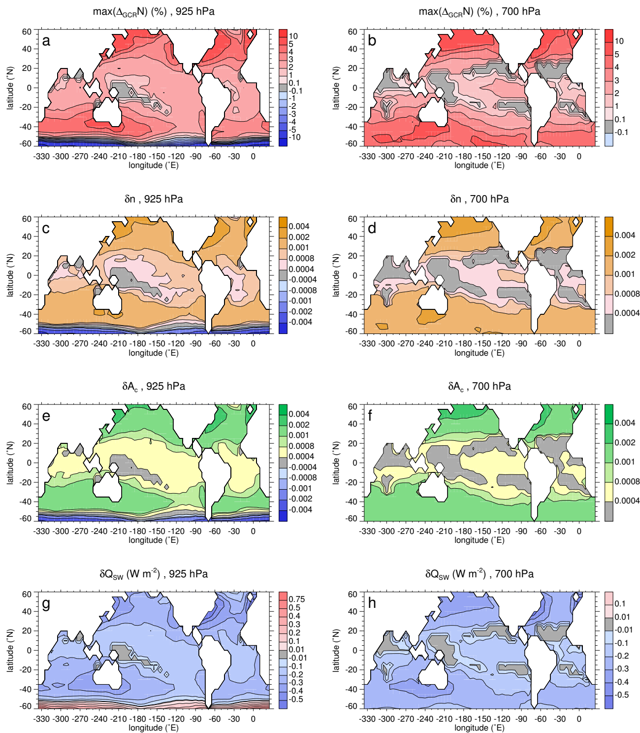
Fig. 12. Spatial distributions of \max(\Delta_{\text{GCR}} N) (a, b), and of the resulting change in cloud fraction \delta n (c, d), cloud albedo \delta A (e, f), and in the daily mean shortwave radiative forcing \delta Q_{\text{SW}} (g, h) for aerosol that nucleated at the 925 hPa (left) and 700 hPa (right) levels, on 21 March.
