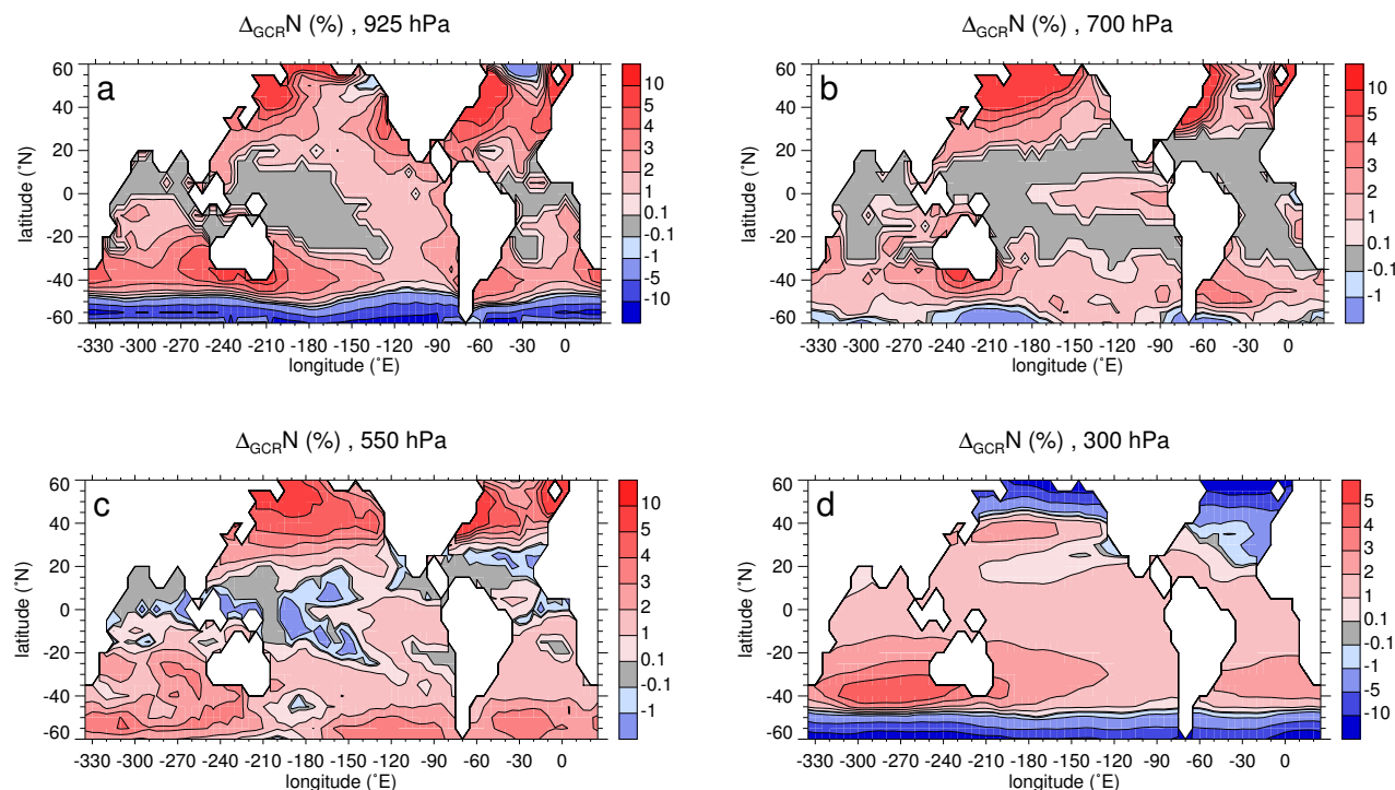
Fig. 7. Response of the supercritical aerosol concentration to the change in GCR ionization from solar maximum to minimum, calculated for noon of 21 March. Areas with \Delta_{\text{GCR}} N > 0 are colored red, areas with \Delta_{\text{GCR}} N < 0 blue. Areas with aerosol concentrations below 0.001 \text{ cm}^{-3} , or where |\Delta_{\text{GCR}} N| < 0.1\% are colored gray.
