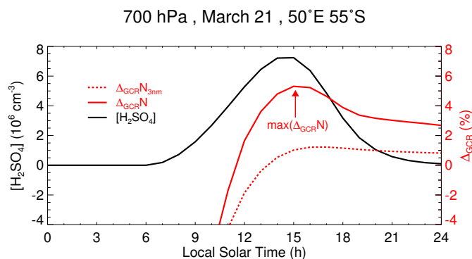
Fig. 8. Gas phase concentration of \text{H}_2\text{SO}_4 for 21 March at 700 hPa, calculated with solar maximum ionization rates, and the response of supercritical aerosol ( \Delta_{\text{GCR}} N ) and of >3 \text{ nm} diameter aerosol ( \Delta_{\text{GCR}} N_{3\text{nm}} ) concentrations to GCR ionization.
