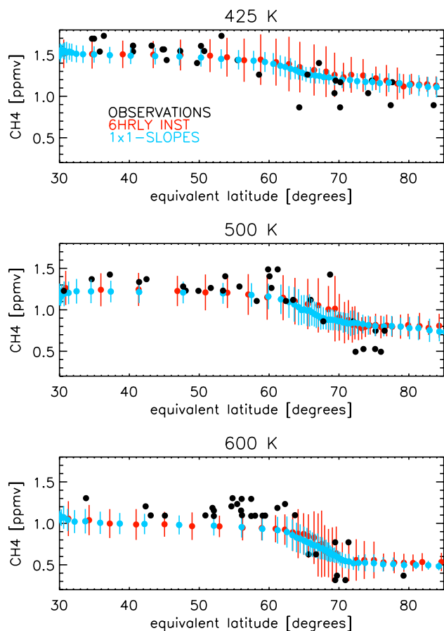
Fig. 6. Similar as Fig. 5, but with the results from the experiments “6-hourly inst.” (red dots) and “ 1\times 1 -slopes” (blue dots).
