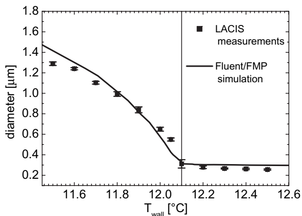
Fig. 4. Measured and simulated droplet diameters at the LACIS outlet for varying wall temperatures, for NaCl particles with a dry diameter of 50 nm.
