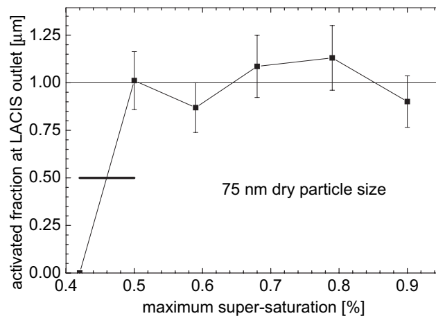
Fig. 7. Measured activated fraction (normalized to one) for the same measurements as shown in Fig. 6. The black bar indicates the uncertainty of the measurement with respect to the super-saturation.
