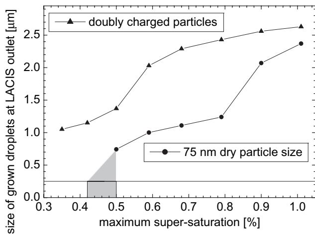
Fig. 6. The size of the droplets grown on 75 nm (and the respective doubly charged 111 nm) urban atmospheric aerosol particles for different super-saturations in LACIS.
