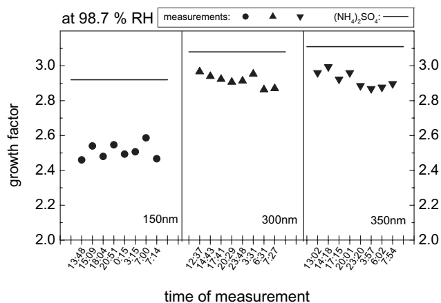
Fig. 11. Similar to Fig. 10, but for 98.7% RH.
