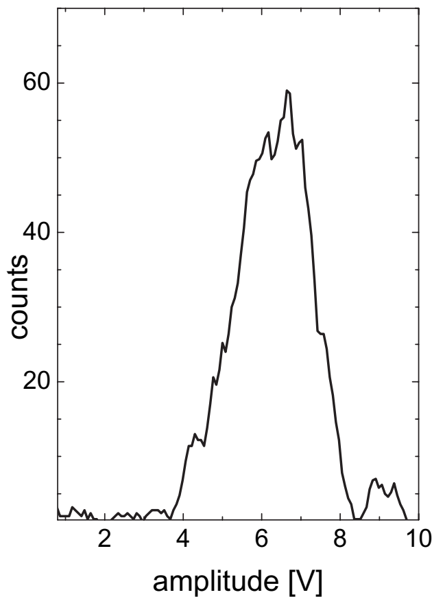
Fig. 3. An exemplary signal measured with the optical particle spectrometer, for the measurement at 11.8°C. Doubly charged particles that passed the DMA appear at a pulse height of about 9 V, clearly distinguished from the main peak.
