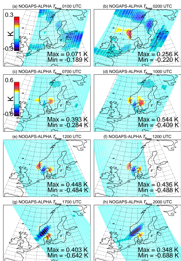
Fig. 16. Similar presentation to Fig. 6, but showing brightness temperature perturbations T'_{B_{\text{NWP}}}(\hat{\lambda}_j, \hat{\phi}_j) derived via Eqs. (2) and (6) from the hourly NOGAPS-ALPHA temperature hindcast field closest in time to the satellite overpass in question. Values are in Kelvin (see color bars): for panels (a) and (b) the range is \pm 0.3 K, whereas for panels (c–h) the color bar range is \pm 0.6 K. Maximum and minimum values for each map are shown in the lower-right portion of each panel.
