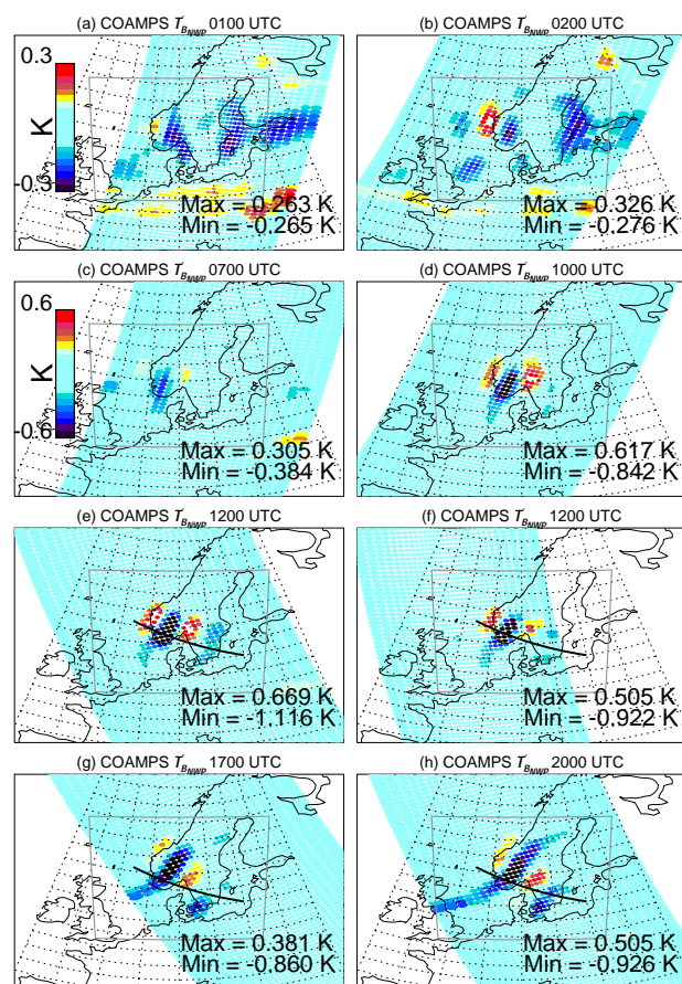
Fig. 17. Same presentation as Fig. 16, but showing brightness temperature perturbations T'_{B_{\text{NWP}}}(\hat{\lambda}_j, \hat{\phi}_j) derived from hourly COAMPS temperature fields. Gray curve shows borders of the COAMPS domain. Black curves in panels (e–h) reproduce the cross section from Figs. 7a and 8 along which brightness temperatures are profiled in Fig. 18.
