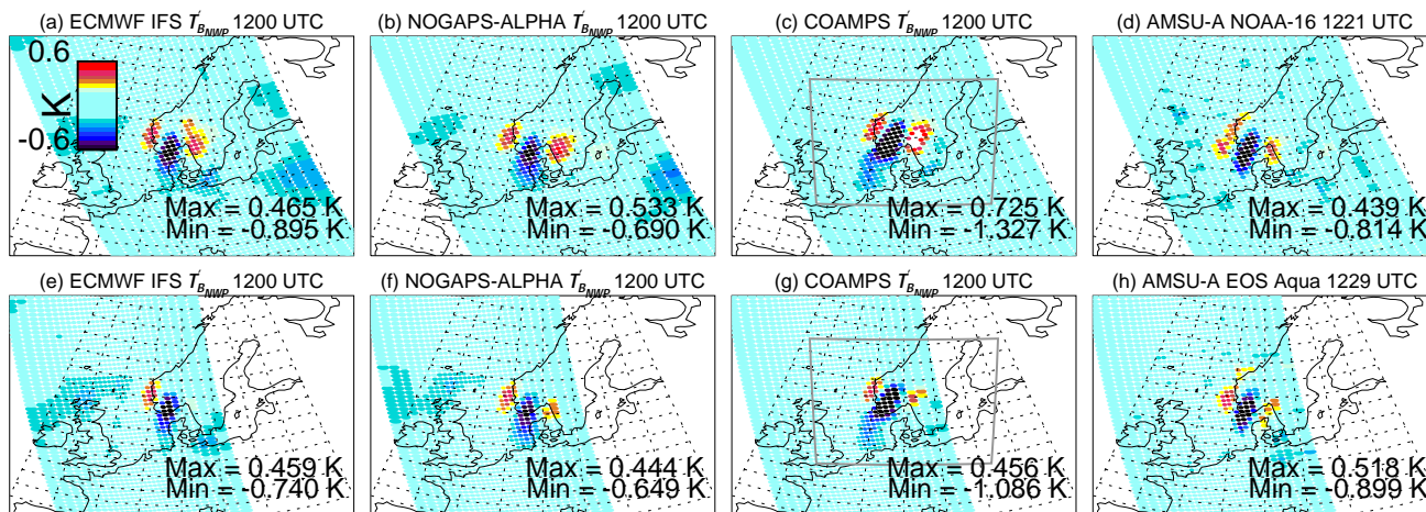
Fig. 14. Top row shows brightness temperature perturbations T'_{B_{\text{NWP}}}(\hat{\lambda}_j, \hat{\phi}_j) computed from Eq. (5) using 12:00 UTC NWP temperature perturbation fields T'(\hat{\lambda}, \hat{\phi}, p) from (a) ECMWF IFS, (b) NOGAPS-ALPHA, and (c) COAMPS runs using AMSU-A scan pattern from the NOAA-16 12:21 UTC overpass. Actual brightness temperatures extracted from these AMSU-A measurements are replotted in (d) from Fig. 6e. Bottom row shows same sequence of plots for the 12:29 UTC EOS Aqua overpass data. Gray borders in (c) and (g) show the regional COAMPS domain. Color bar scale ( \pm 0.6 K) is given at the top-left of panel (a). Maximum and minimum values for each map are shown in the lower-right portion of each panel.
