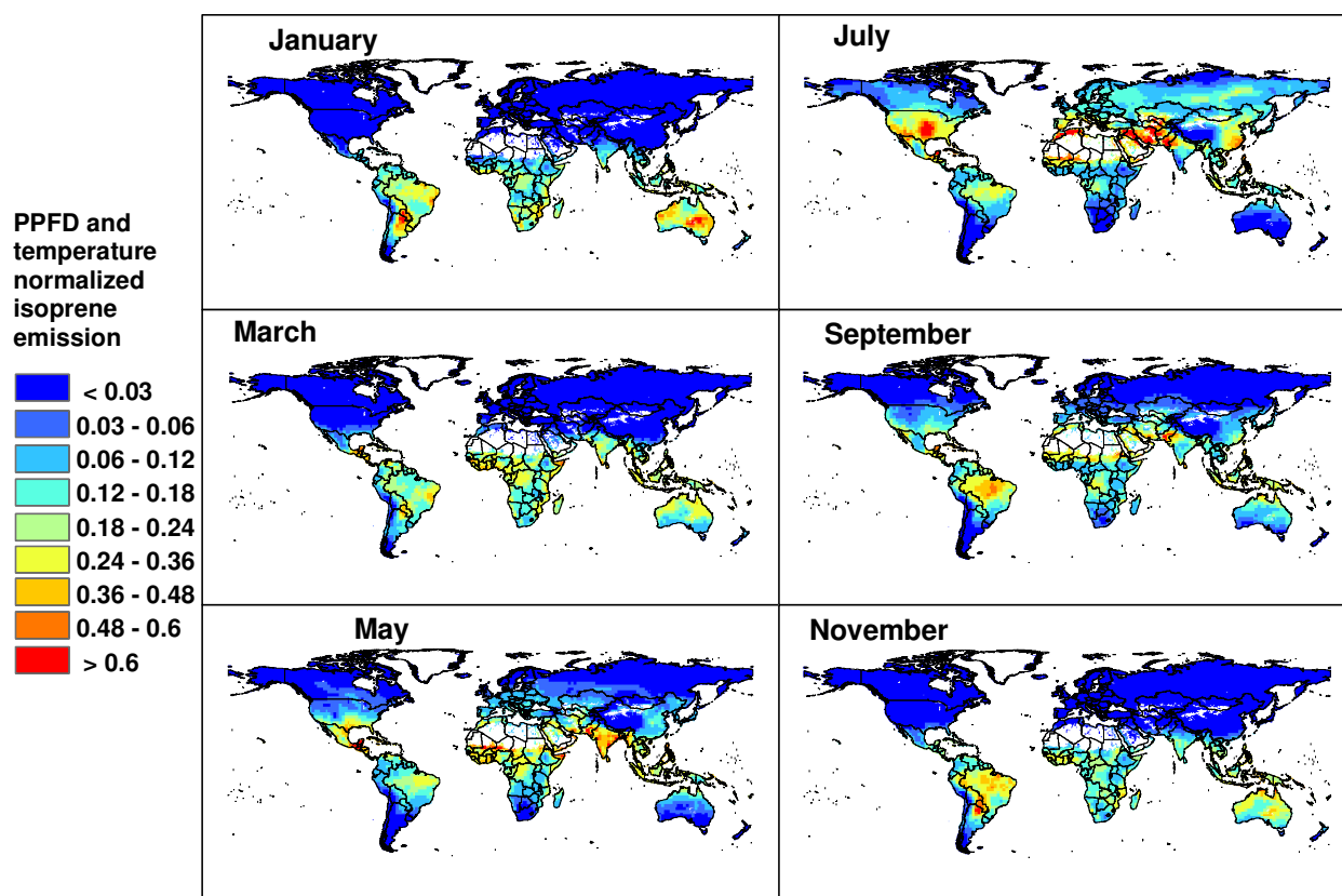
Fig. 9. Monthly normalized isoprene emission rates estimated with MEGAN for 2003. Rates are normalized by the emission estimated for standard temperature ( =303\text{ K} ) and PPFD transmission (60%). These normalized rates illustrate the variations associated with changes only in temperature and PPFD transmission; i.e. all other model drivers are held constant.
