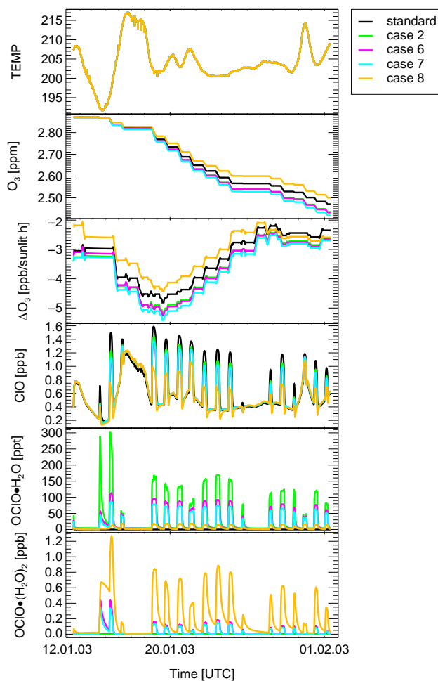
Fig. 8. Temperature, \text{O}_3 , ClO, \text{OCIO}\cdot\text{H}_2\text{O} , and \text{OCIO}\cdot(\text{H}_2\text{O})_2 mixing ratios as well as the ozone depletion per sunlight hour are shown along one Match trajectory starting in mid-January until the beginning of February 2003 for different sensitivity studies considering the \text{OCIO}\cdot(\text{H}_2\text{O})_2 complex chemistry in model simulations.
