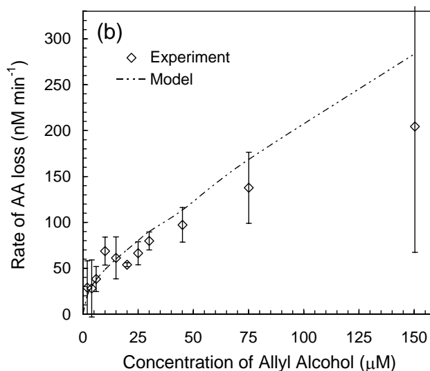
Fig. 5. (a) Rates of 3-bromo-1,2-propane-diol (3BPD) and 3-chloro-1,2-propanediol (3CPD) formation ( R_F^{3\text{BPD}} and R_F^{3\text{CPD}} ) as a function of [\text{AA}] in illuminated (313 nm) aqueous halide solutions ( [\text{Cl}^-]=0.56\text{ M} , [\text{Br}^-]=0.80\text{ mM} , and pH 3.0) containing 1.0 mM \text{H}_2\text{O}_2 . The symbols and error bars are the same as in Fig. 3a. (b) Rates of allyl alcohol loss ( R_L^{\text{AA}} ) in the experiments described in Fig. 5a. The symbols and error bars are the same as in Fig. 3b.
