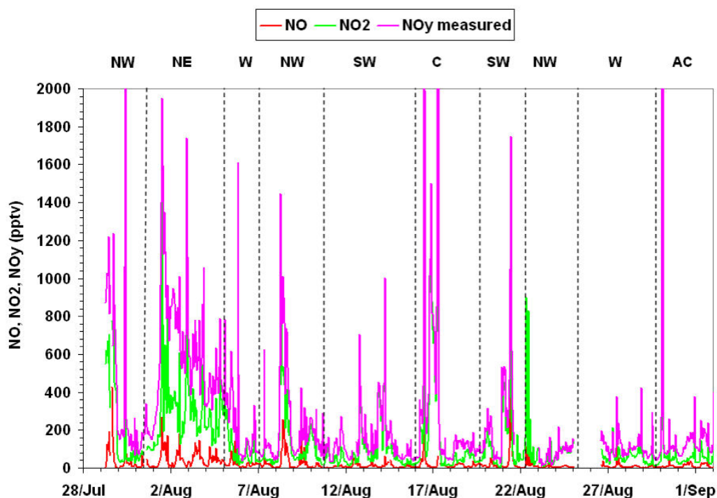
Fig. 10. Time-series of NO, NO 2 , and measured NO y .
