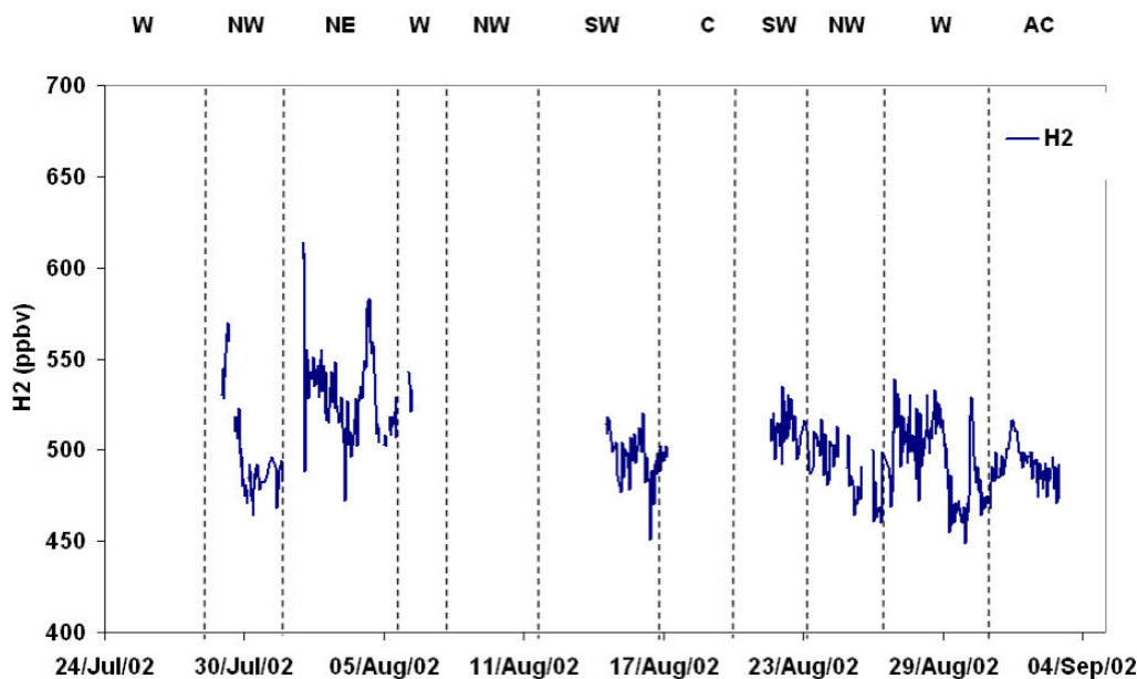
Fig. 7. Time-series for hydrogen at Mace Head during NAMBLEX.
