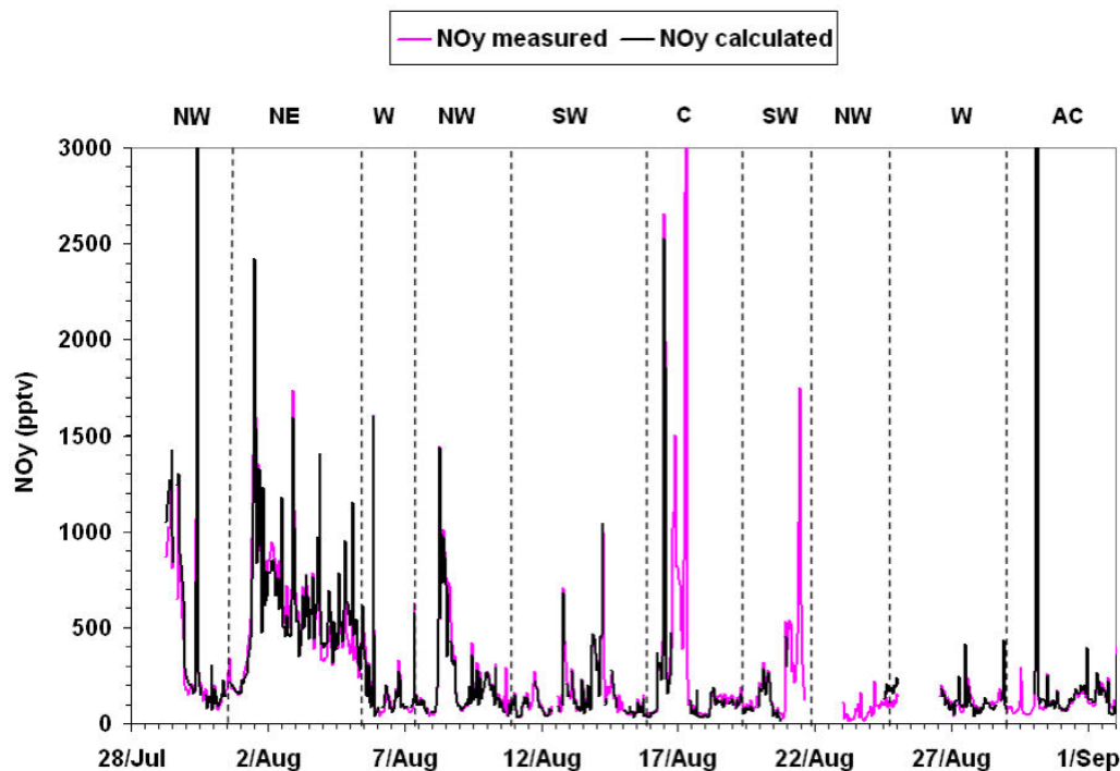
Fig. 11. Time-series of measured and calculated NO y , the latter by summing the measured NO, NO 2 , HNO 3 , PAN and organic N.
