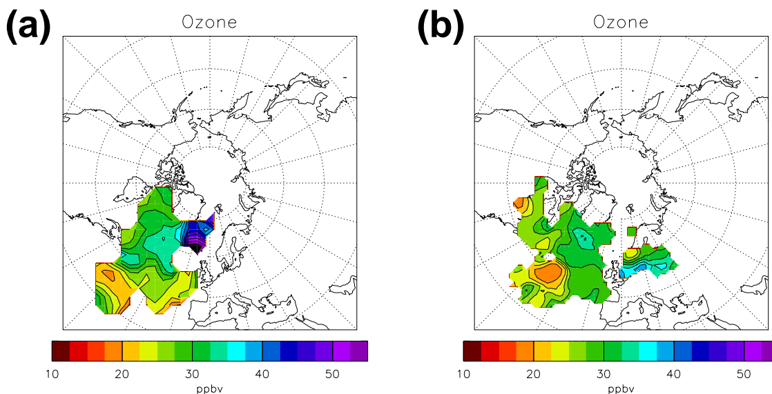
Fig. 21. Map of origin-averaged ozone. Plots showing average ozone data (DEFRA) for every hour during EASE96 on lefta and NAMBLEX on rightb which are used to label the origin of the 5 day back trajectory from Mace Head.
