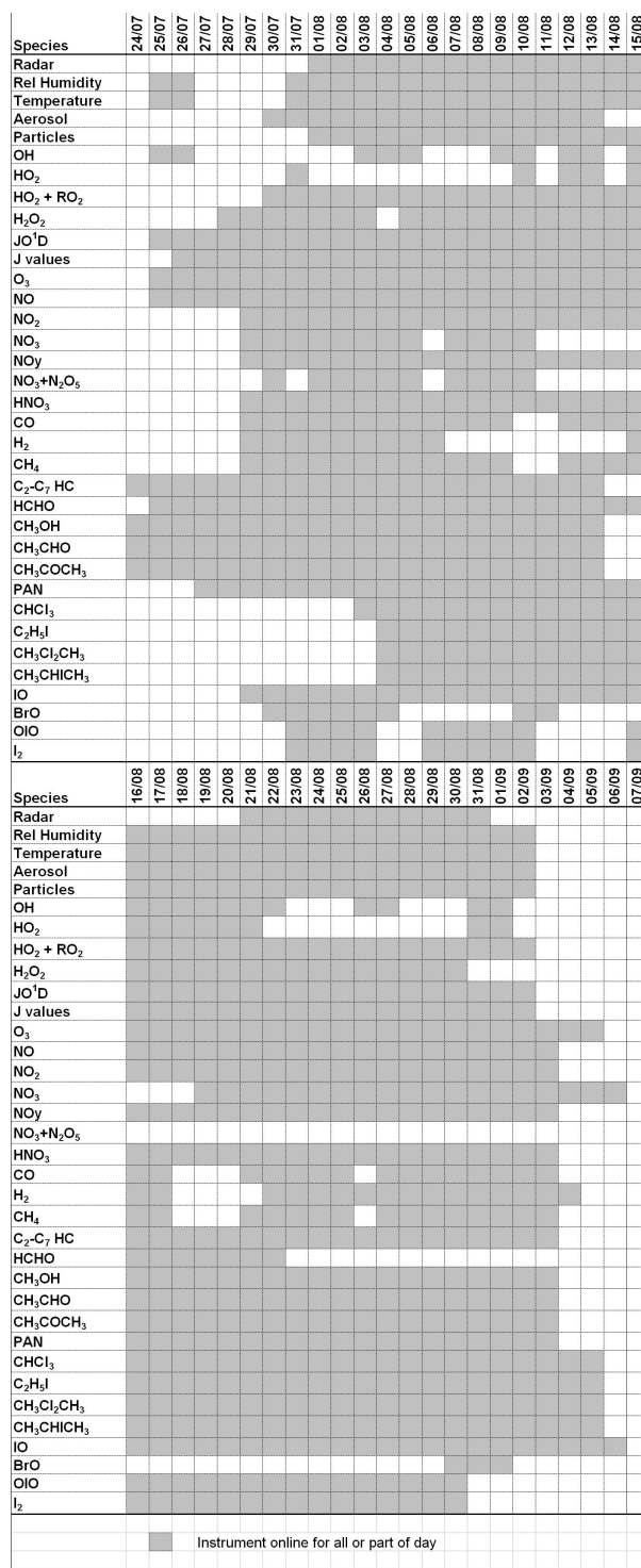
Fig. 3. Time-line showing data coverage for the NAMBLEX campaign, 2002.
