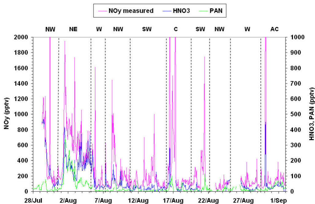
Fig. 12. Time-series of measured \text{NO}_y , \text{HNO}_3 , and PAN.
