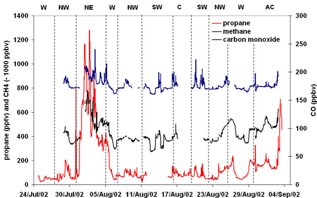
Fig. 8. Time-series of methane, propane and carbon monoxide.
