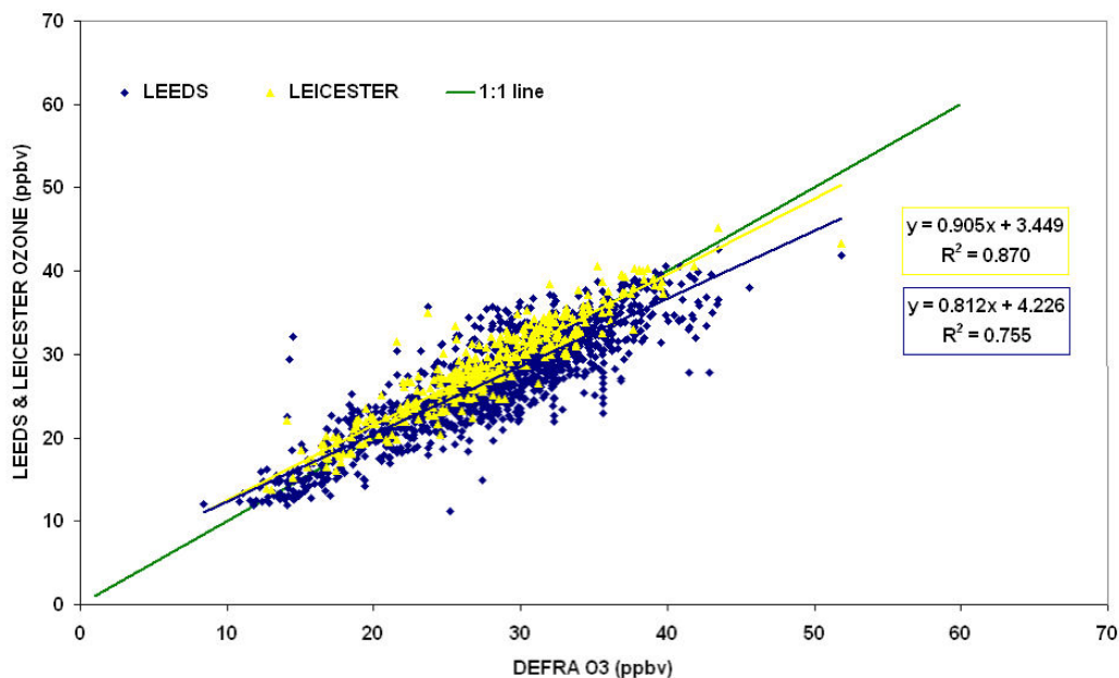
Fig. 5. Correlation of all O_3 measurements made during NAMBLEX at Mace Head.
