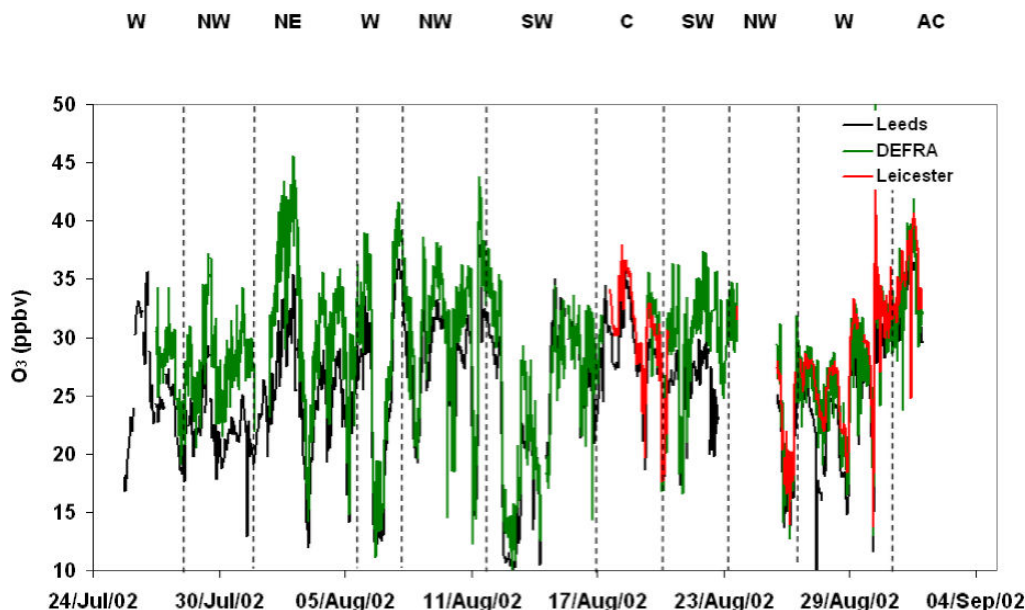
Fig. 4. Time-series of 30-min averaged O_3 . W = West, NW = Northwest, NE = Northeast, SW = Southwest, C = Cyclonic, AC = Anticyclonic.
