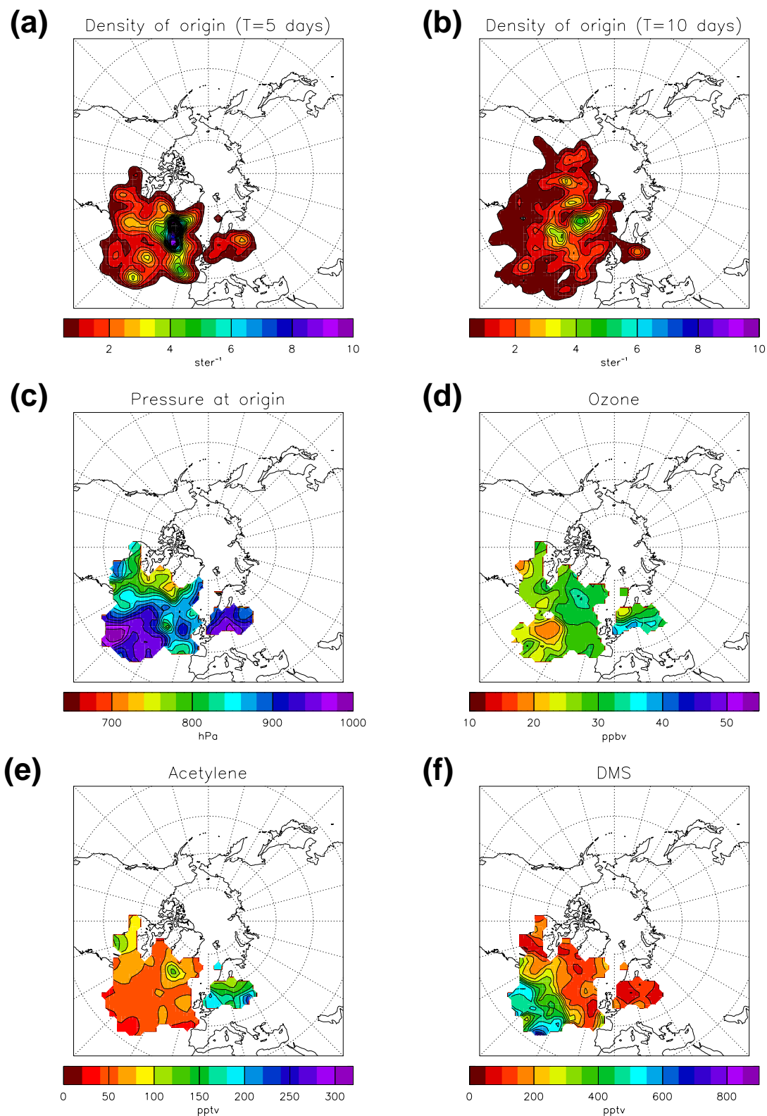
Fig. 16. (a): Density of origin plot for 5-day back trajectories from 500 m above Mace Head during NAMBLEX, (b): As (a) but for 10 days, (c): Origin-averaged pressure at origin of air mass, (d): Origin-averaged ozone, (e): Origin-averaged acetylene, (f): Origin-averaged DMS. (c–f based on 5-day trajectories).
