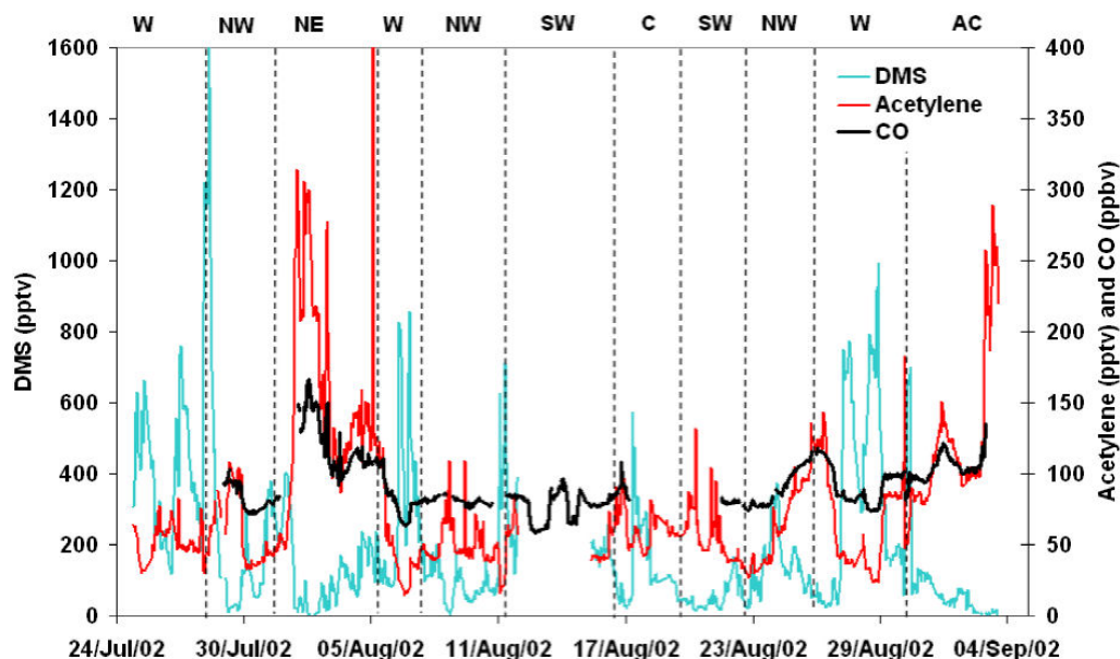
Fig. 6. Time-series of carbon monoxide, acetylene and dimethyl sulfide.
