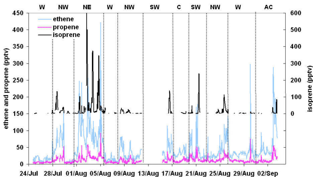
Fig. 9. Time-series of ethene, propene, and isoprene (vertically displaced for clarity).
