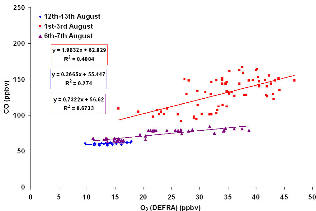
Fig. 20. CO versus O 3 for a “polluted” period (1–3 August in red) a “clean” westerly period (6–7 August in purple), and for a “cleaner” south westerly period (12–13 August in blue) during NAMBLEX 2002.
