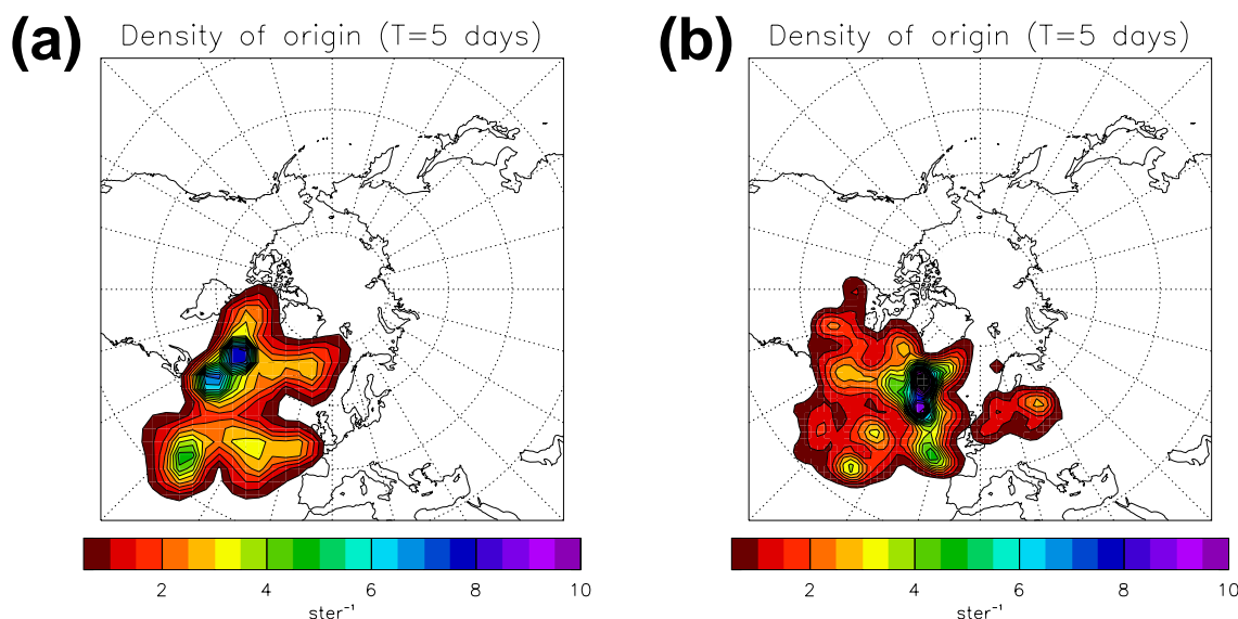
Fig. 19. Density of origin plots using 5-day back trajectories for EASE96 (left) (a) and NAMBLEX (right) (b).
