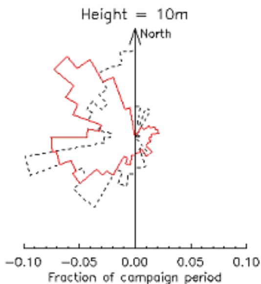
Fig. 15. Wind Rose showing the frequency of different wind directions for the local measurement from the met mast (red) and for the ECMWF analyses at 10 m (dashed).
