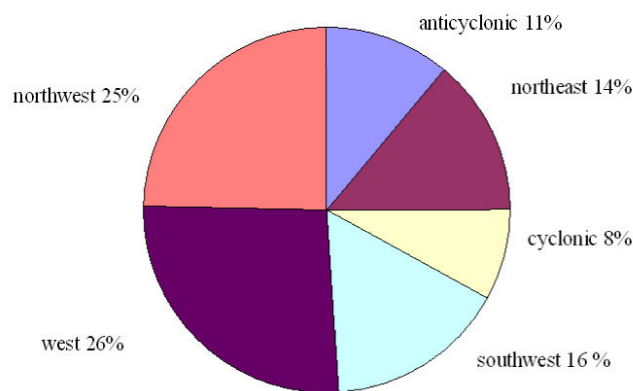
Fig. 18. The distribution of trajectory classifications during NAMBLEX.
