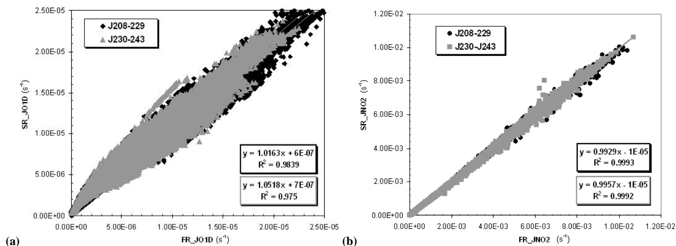
Fig. 13. (a): Correlation plot for j(\text{O}^1\text{D}) measured using the University of Leicester's filter radiometer (FR) and diode array spectroradiometer (SR). (b): Correlation plot for j(\text{NO}_2) measured using the University of Leicester's filter radiometer (FR) and diode array spectroradiometer (SR). The two Julian day ranges refer to data from the first and second halves of the campaign, respectively.
