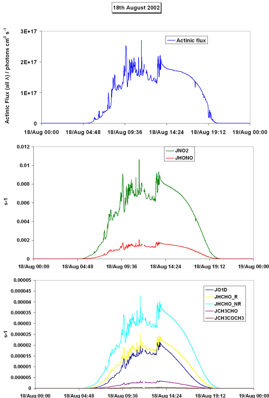
Fig. 14. (a): Actinic flux, (b): j -(NO 2 ) and j -(HONO), (c): j -(O 1 D), j -(HCHO)NR (non-radical, HCHO+hν→H 2 +CO), j -(HCHO)R(radical, HCHO+hν→HCO+H→HO 2 +HO 2 +CO), j -(CH 3 CHO), and j -(CH 3 COCH 3 ) for a clean day 18 August 2002.
