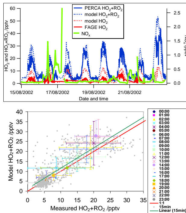
Fig. 4. (a) Measured and modelled PERCA [\text{HO}_2 + \Sigma \text{RO}_2] and FAGE [\text{HO}_2] ; (b) MCM modelled vs. measured [\text{HO}_2 + \Sigma \text{RO}_2] (15 min data) and hourly-averaged data.
