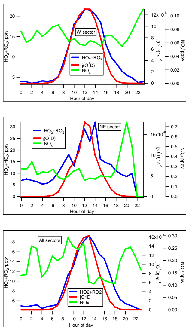
Fig. 3. Hourly-averaged [\text{HO}_2 + \Sigma \text{RO}_2] , [\text{NO}_x] and j(\text{O}^1\text{D}) diurnal cycles for all campaign data and W and NE air-mass sector data subsets.
