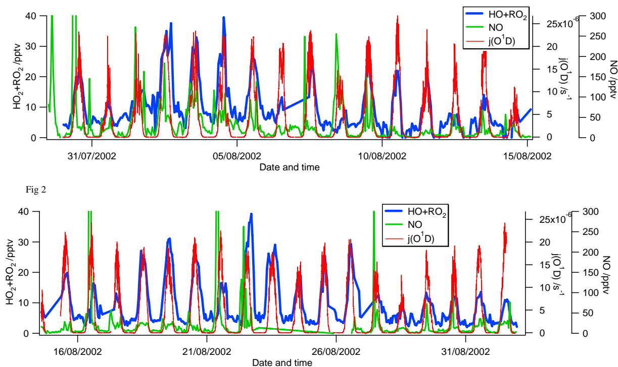
Fig. 2. [HO 2 + ΣRO 2 ], j (O 1 D) and [NO] campaign time series.
