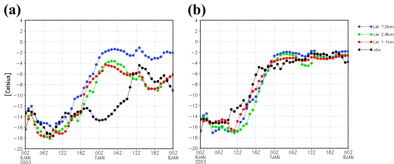
Fig. 10. Time series of 2 m temperature [ ^{\circ}\text{C} ] for LM 7.0 km, 2.8 km, 1.1 km and observations, 48 h forecast of 06 January 2003, 00:00 UTC. (a) Blindern, (b) Tryvann.
