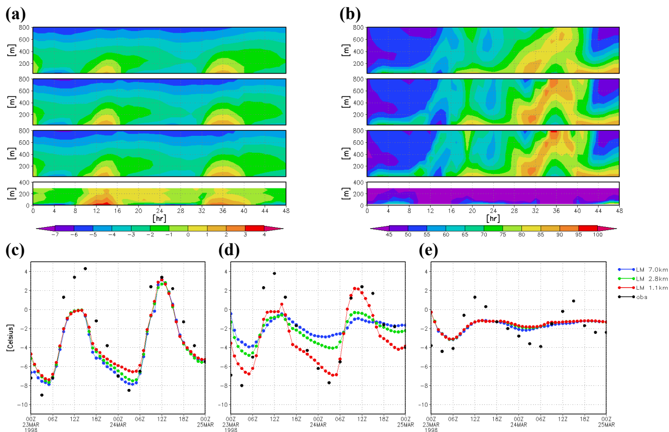
Fig. 7. LM 48 h forecasts for 7.0 km, 2.8 km, 1.1 km resolution starting 23 March 1998, 00:00 UTC, and observations. Top: Vertical profiles as 48 h time series for (a) temperature [ ^{\circ}\text{C} ] and (b) relative humidity [%] (top to bottom: 7.0 km, 2.8 km, 1.1 km, observations). Bottom: 48 h time series of 2 m temperature [ ^{\circ}\text{C} ] for (c) Vantaa, (d) Kaisaniemi, (e) Isosaari.
