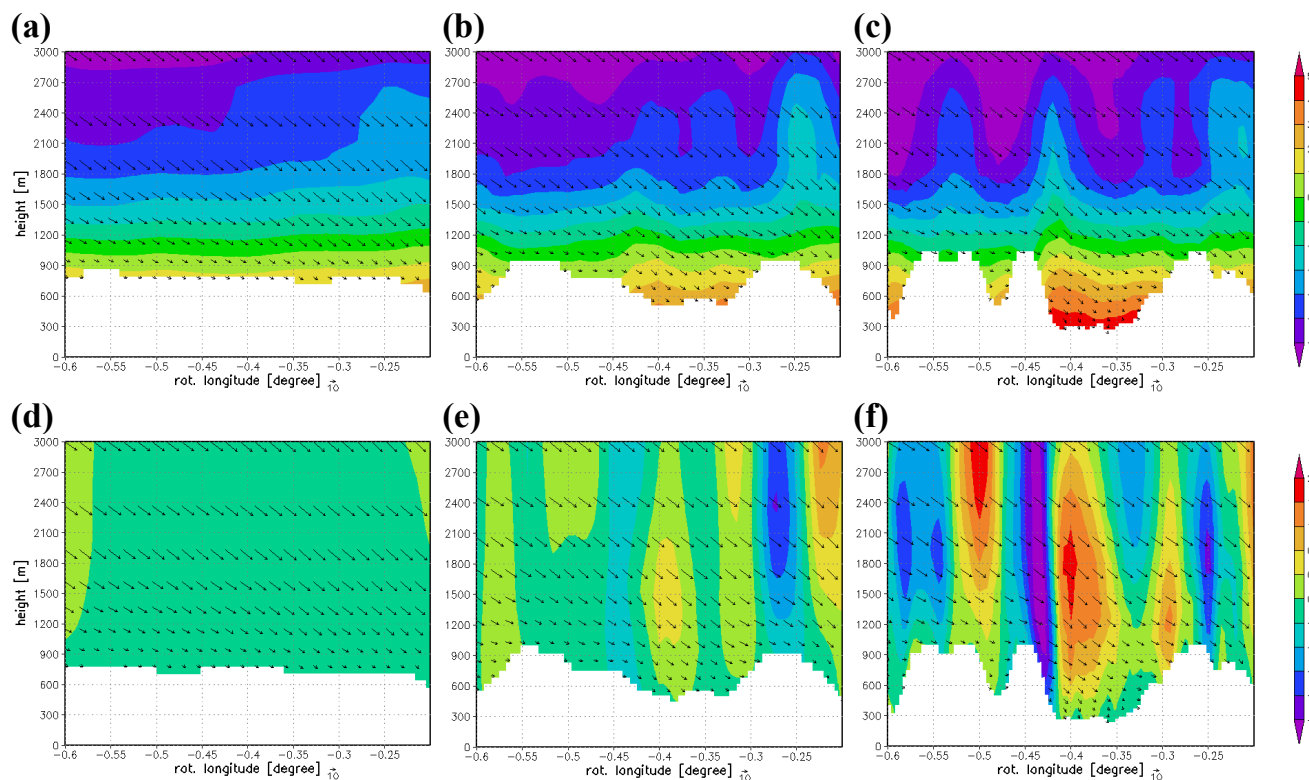
Fig. 9. Oslo forecasts with LM of 7, 2.8, 1.1 km resolution, 17 November 2001, 00:00 UTC +18 h. Vertical cross section along Hallingdal valley with horizontal wind speed and direction (black arrows) and shaded (a–c) temperature [ ^{\circ}\text{C} ], (d–f) vertical velocity [m/s].
