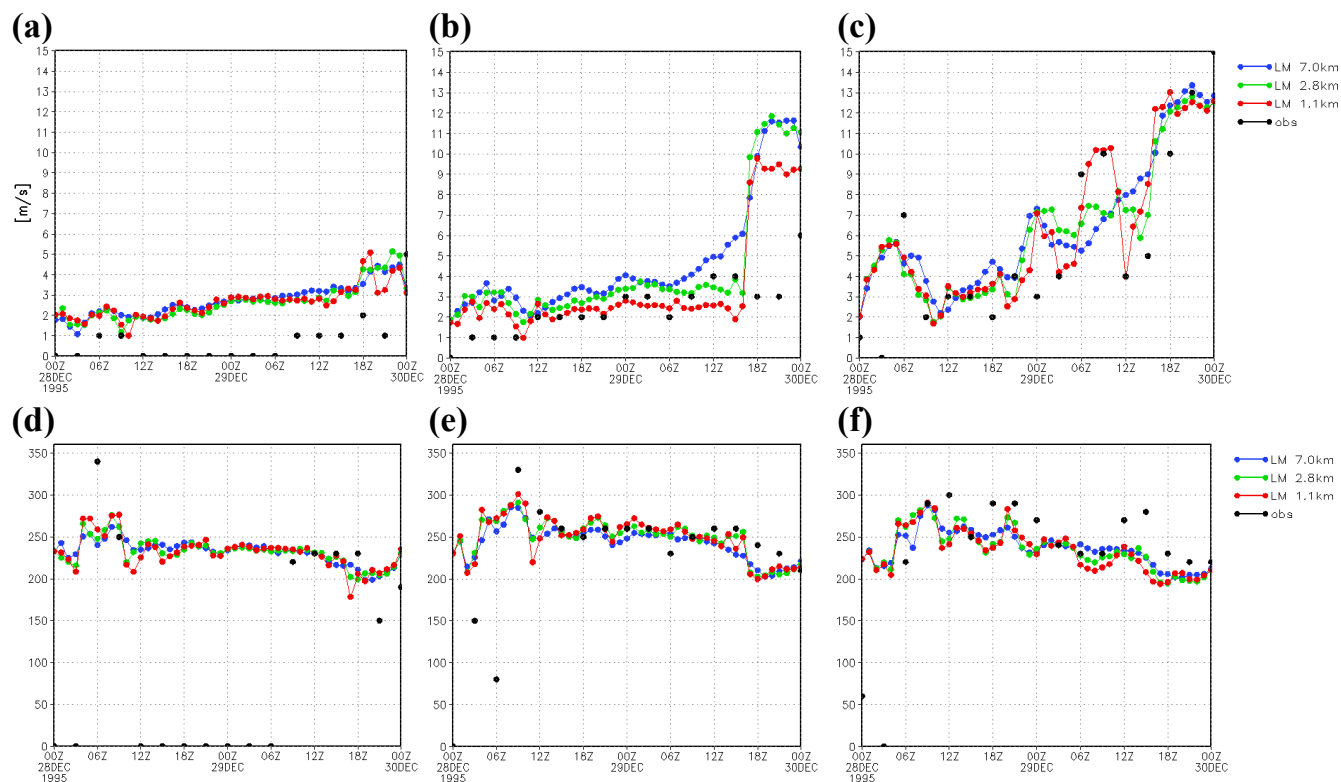
Fig. 6. Time series of 10 m horizontal wind fields for 48 h LM forecasts for 7.0 km, 2.8 km, 1.1 km resolution starting 28 December 1995, 00:00 UTC, top: wind speed [m/s] for (a) Vantaa, (b) Kaisaniemi, (c) Isosaari, and bottom: wind direction for (d) Vantaa, (e) Kaisaniemi, (f) Isosaari.
