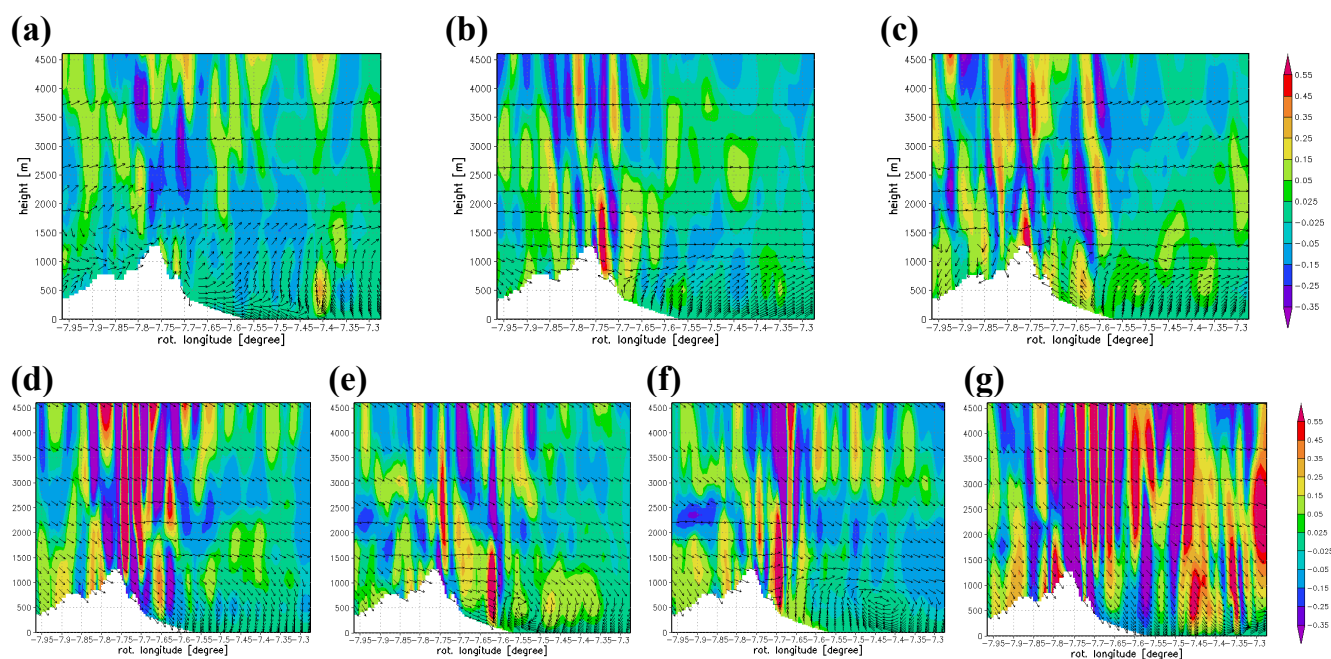
Fig. 12. Vertical cross section perpendicular to Mediterranean coast north of Valencia (height [m] vs. LM rotated geographical longitude [ ^{\circ} ]) for vertical velocity [m/s] (shaded contours) and horizontal wind vector (arrows) for 1.1 km LM forecasts, (a) 27 September 1999, 00:00 UTC +3 h, (b) 27 September 1999, 00:00 UTC +10 h, (c) 27 September 1999, 00:00 UTC +13 h, (d) 28 September 1999, 00:00 UTC +10 h, (e) 28 September 1999, 00:00 UTC +13 h, (f) 28 September 1999, 00:00 UTC +14 h, (g) 30 September 1999, 00:00 UTC +14 h.
