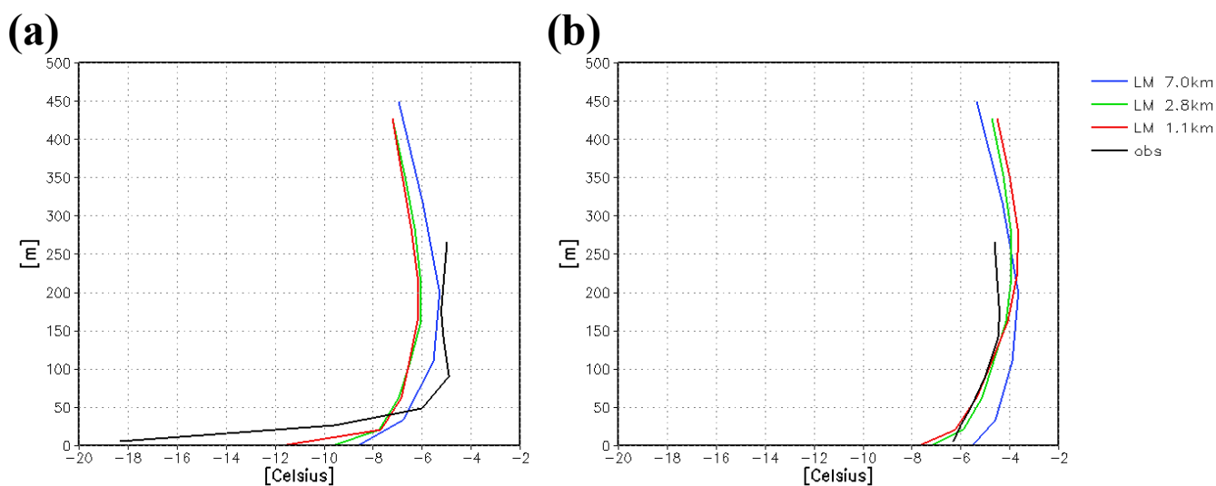
Fig. 3. Vertical profiles of forecast temperature [ ^{\circ}\text{C} ] for LM 7.0 km, 2.8 km, 1.1 km grid resolution for Kivenlahti mast including observations on 28 December 1995, 00:00 UTC (a) +6 h and (b) +36 h.
