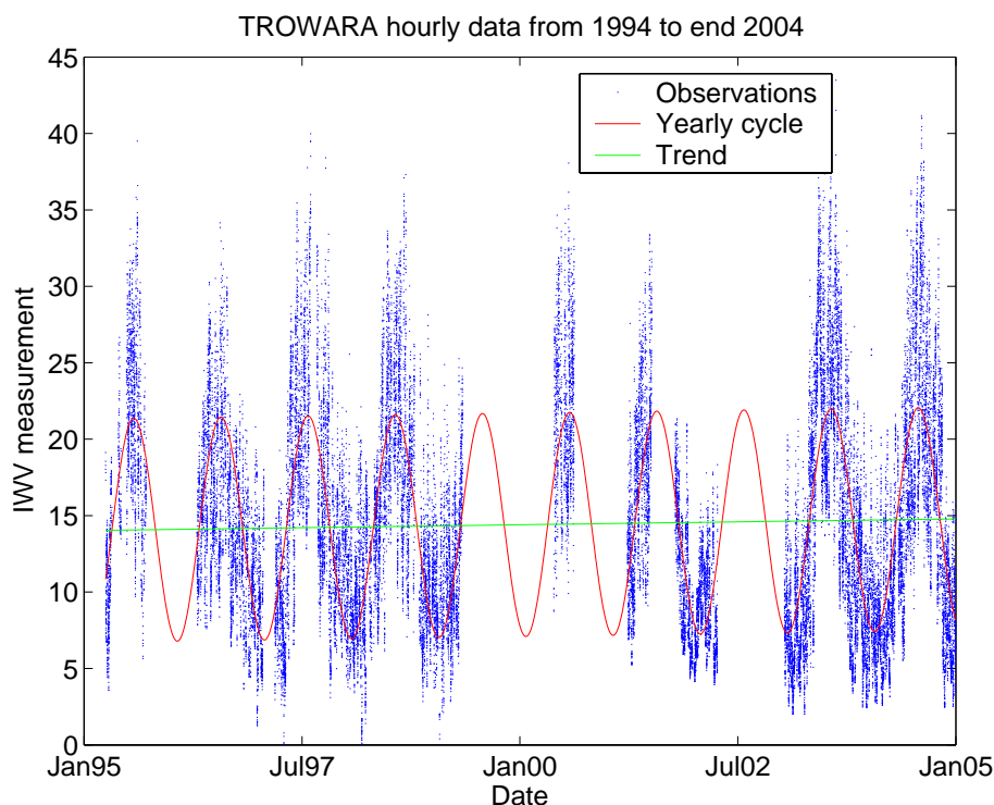
Fig. 3. Time series of TROWARA hourly integrated water vapour (IWV) measurements (blue points) with a model of the annual cycle (red) and trend (green). Units are \text{kg}/\text{m}^2 .
