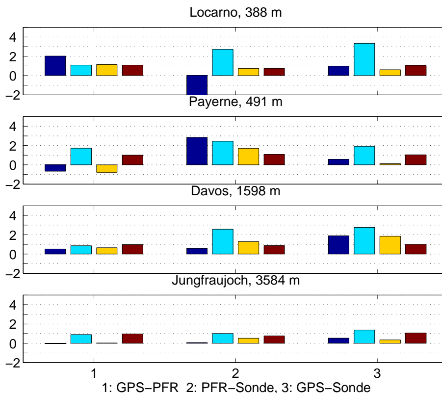
Fig. 10. The bias (light blue), standard deviation (dark blue), intercept (yellow) and slope (brown) of the relationships between IWV measurements made at Locarno, Payerne, Davos and Jungfrauoch. Units are \text{kg}/\text{m}^2 . The comparisons between GPS (dependent) and PFR (independent), PFR (dependent) and radiosonde (independent) and GPS (dependent) and radiosonde (independent) are shown in the first, second and third sets of bars, respectively. The radiosonde measurements are integrated from the height of the station used in the comparison.
