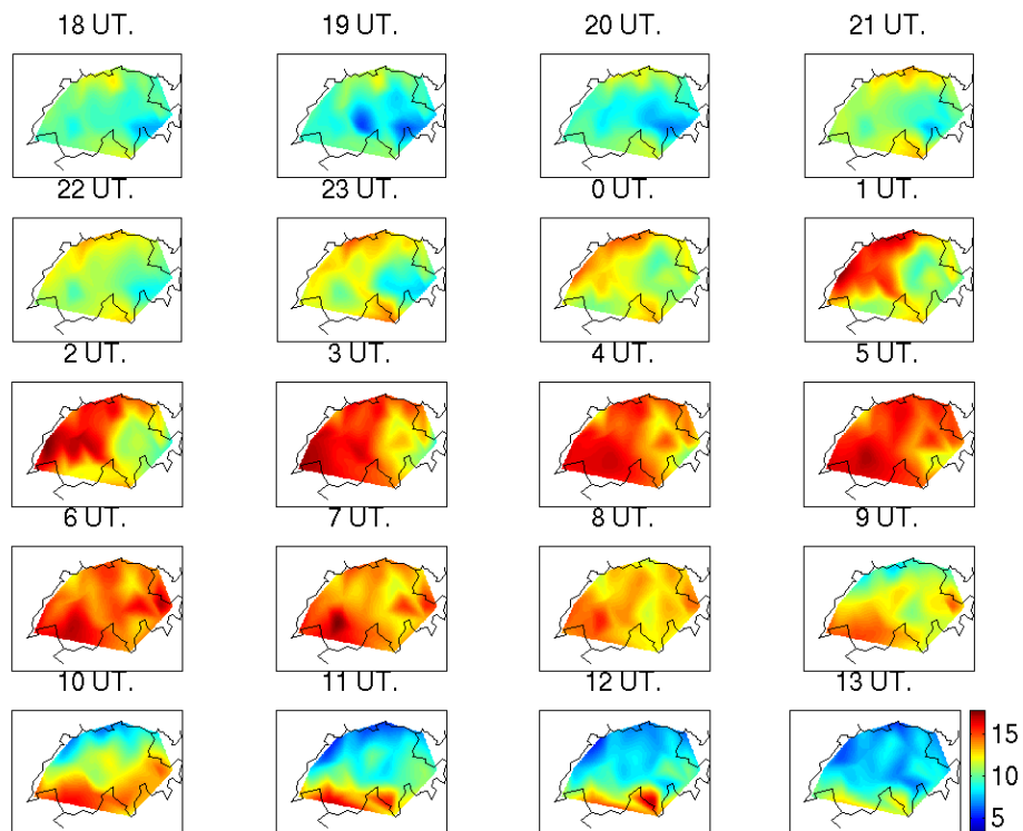
Fig. 12. The IWV measured by the GPS network during the passage of a frontal system from 18:00 UT on 18 November 2004 to 13:00 UT on the 19 November 2004. Units are \text{kg}/\text{m}^2 . The IWV for all stations is corrected to a height of 500 m. The plots represent GPS measurements from the previous hour and are shown at hourly intervals.
