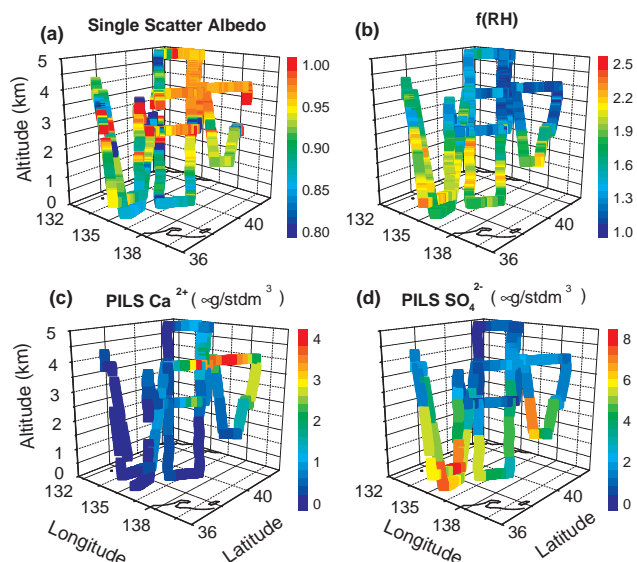
Fig. 4. Typical spatial scales, variability and coupling between aerosol optical properties and related chemical signatures are shown for data collected during ACE-Asia aboard the NSF/NCAR C-130 (Anderson et al., 2003; Clarke et al., 2004; Lee et al., 2003). This flight path for 8 April 2001 represents a box approximately 400 km square and 5 km. Dust outflow at larger altitudes to the north is evident from the aerosol exhibiting large single scattering albedo (a), a low humidity dependence of the scattering coefficient f\sigma_{sp}(80, 40) (b), and large calcium concentrations (c). Combustion derived aerosols near the surface to the south are evident from the large concentrations of sulfate (d) and consequent large values of f\sigma_{sp}(80, 40) (b). These aerosols also contain large concentrations of black carbon (not shown) which result in small single scattering albedo values (a). The concentrations of ionic species were measured with a particle-into-liquid sampler (PILS) and ion chromatograph. The species mixing ratios are given at 1 atmosphere and 25°C.
