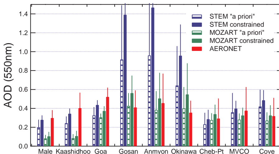
Fig. 24. Test of model ability to reproduce measured aerosol optical depth at 550 nm ( \tau_{550} ). The test is based on diurnal-mean data at nine AERONET stations (three from each region, all located on either islands or coasts) and for the model grid cells containing those stations. NIO stations include: Male ( 4.2^\circ N, 73.5^\circ E, 2 m elevation), Kaashidoo ( 5.0^\circ N, 73.5^\circ E, 0 m), and Goa, India ( 15.5^\circ N, 73.8^\circ E, 20 m). NWP stations include: Gosan ( 33.3^\circ N, 126.2^\circ E, 0 m), Anmyon ( 36.3^\circ N, 126.2^\circ E, 47 m), and Okinawa ( 26.4^\circ N, 127.8^\circ E, 46 m). NWA stations include: Chebogue Pt. ( 43.7^\circ N, 66.1^\circ W, 0 m), Martha's Vineyard Coastal Observatory ( 41.3^\circ N, 70.6^\circ W, 10 m), and Cove Lighthouse ( 36.9^\circ N, 75.7^\circ W, 37 m). Bar height denotes campaign-wide means and whisker standard deviations at each station for the four types of model and for the AERONET measurements. The number of days with STEM and MOZART data at each station N is indicated below the station name. Further details on the analysis method and test results are given in the text, Sect. 5.4, and Table 26. Note that sea salt hygroscopic growth was held at 80% RH in the model runs.
