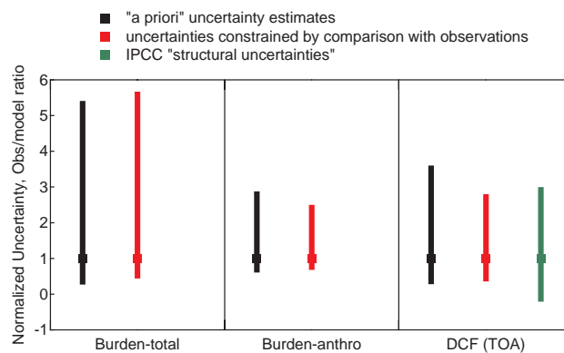
Fig. 28. Normalized uncertainties (uncertainty range of the indicated quantity divided by the value of the quantity) associated with the mean total aerosol column burden, the mean anthropogenic aerosol column burden, and the aerosol direct climate forcing (DCF), for the northwest Pacific region during ACE-Asia. Also shown for comparison is the normalized uncertainty associated with the global mean aerosol direct climate forcing calculated (Table 28; Fig. 26) from IPCC (Ramaswamy et al., 2001) estimates of the uncertainties in the forcings by the several aerosol species; negative value indicates that the uncertainty range of this (negative) forcing encompasses values of opposite sign (i.e., positive).
