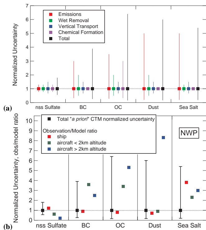
Fig. 27. (a) Normalized uncertainties (uncertainty range of the indicated quantity divided by the value of the quantity) associated with the CTM (Table 19) in the NWP. (b) Total normalized uncertainty in the “a priori” CTM calculations (from Fig. 27a) compared with the ratio of the mean CTM calculated concentration to the measured concentration along the Ronald H. Brown cruise track during ACE-Asia (Table 20) and the C-130 flight track during ACE-Asia.
