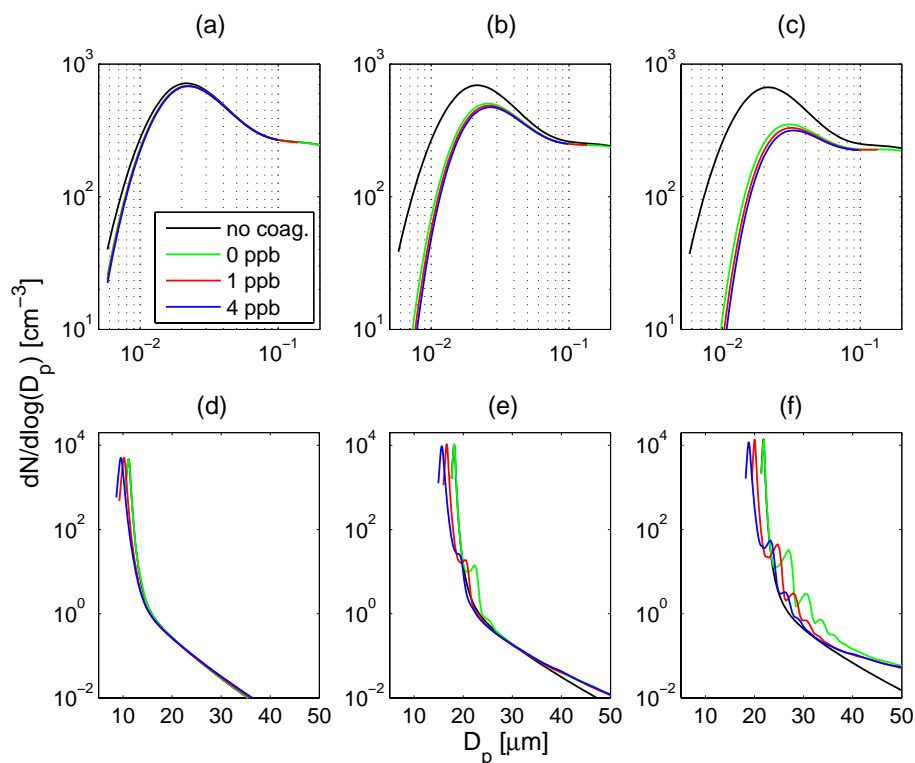
Fig. 4. Interstitial aerosol particles (a, b, c) and cloud droplets (d, e, f) 100 s (a, d), 500 s (b, e) and 900 s (c, f) after cloud formation. For reference, curves without coagulation (0 ppb of HNO 3 ) and with coagulation for 0 ppb, 1 ppb and 4 ppb of HNO 3 are presented. The initial size distribution is continental from Table 1.
