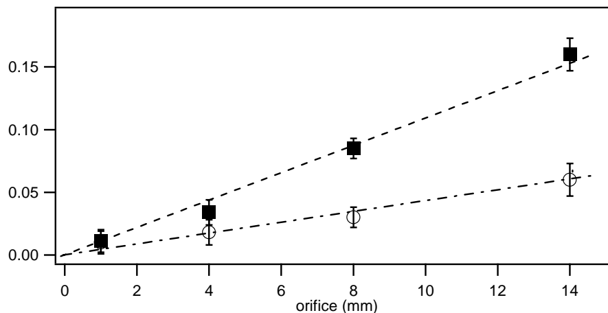
Fig. 3. Dependence of \gamma_0 (full squares) and \gamma_{ss} (open circles) for the uptake of N 2 O 5 on 580 mg CaCO 3 powder on orifice size: A_s is 4.9 cm 2 , F_0^{N_2O_5}=2.3 \times 10^{15} molecule s -1 .
