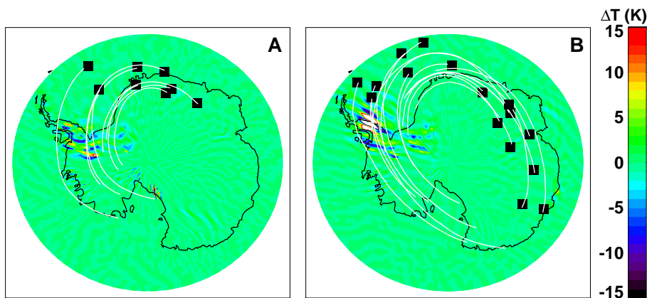
Fig. 4. Colour-coded MWMF-3 hindcast mountain-wave temperature perturbations for 12:00 UT on 10 June (A) and 12:00 UT on 11 June (B). Overlaid backward trajectories (white lines) start at the times and locations of MIPAS NAT observations (squares) on 11 June (A) and 12 June (B) and end at 00:00 UT on 10 June (A) and 00:00 UT on 11 June (B). Note that the MWMF-2 solutions in Fig. 3 show peak wave amplitudes only, whereas the MWMF-3 runs in this figure provide both amplitude and phase.
