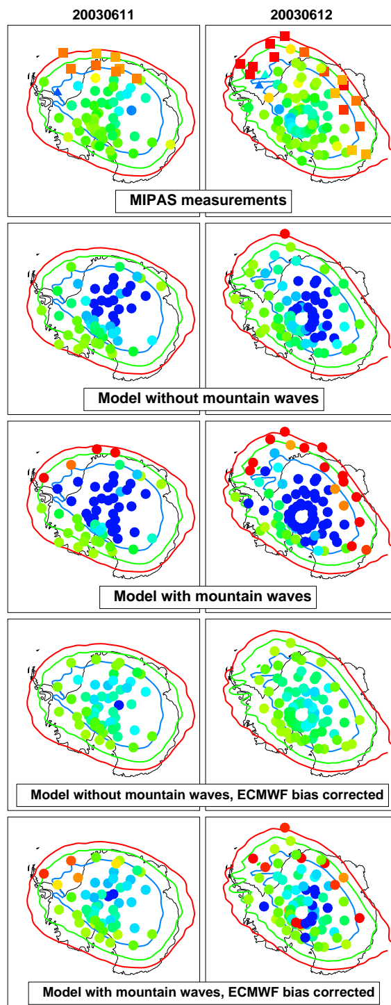
Fig. 5. MIPAS measurements on 11 and 12 June in comparison with DMI microphysical PSC box model simulations at the time and location of the observations. The colour scale is the same as in Fig. 2. In the 2nd row the ECMWF temperatures are used, whereas model runs shown in the 3rd row add the mountain wave corrections from MWFM-3. Rows 4 and 5 show equivalent runs, but on basis on ECMWF temperatures which have been corrected for a bias with respect to radiosondes (see text).
