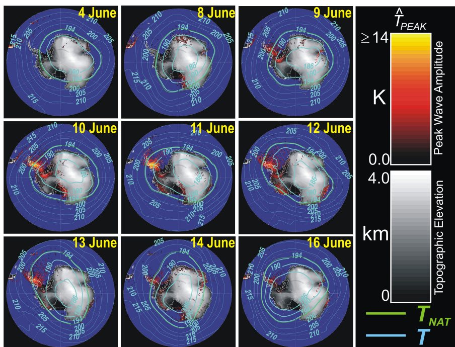
Fig. 3. MWMF-2 hindcast of peak mountain wave temperature amplitudes at 40 hPa for various days in June 2003 at 12Z, based on 1.25^\circ \times 1^\circ 36-level analyses from NASA's Global Modeling and Assimilation Office. Blue contours show synoptic temperatures, green contour shows the local NAT formation temperature based on a calculation using 10 ppbv of \text{HNO}_3 and 5 ppmv of \text{H}_2\text{O} .
