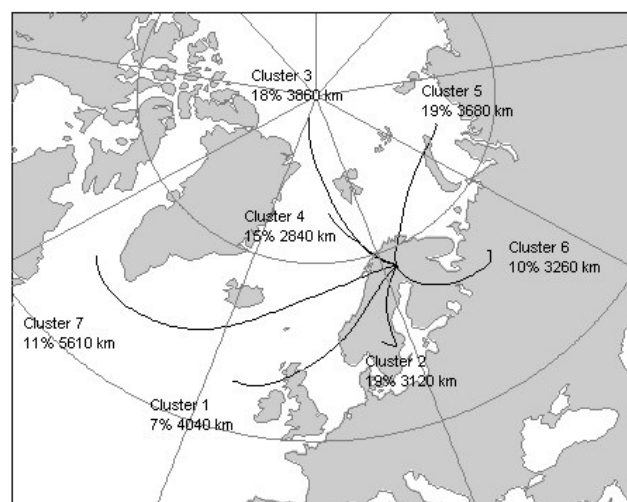
Fig. 8. Transport paths to Pallas illustrated by cluster mean trajectories, denoted 1–7. Percent occurrence of trajectories within each cluster as well as the average trajectory lengths in the different clusters are indicated in the figure.
