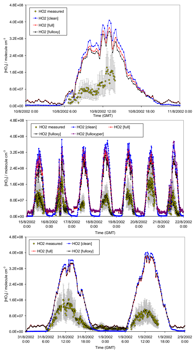
Fig. 3. Model-measurement comparison for HO 2 with the base models. (a) 10 August, (b) 15–21 August, (c) 31 August–1 September. The measurements 2σ standard deviation is shown in grey.
