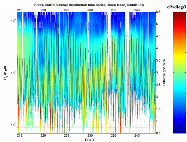
Fig. 5. DMPS particle size distribution series together with tidal height. Note that the unit of the colour-coded bar is an exponential.
