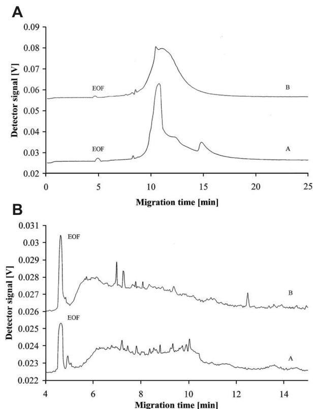
Fig. 5. (a) Electropherograms of Nordic River humic acid in 6 mM \text{Na}_2\text{B}_4\text{O}_7 \cdot 10\text{H}_2\text{O} -3 mM \text{KH}_2\text{PO}_4 , pH=9.00 (trace marked A) and in 5 mM \text{NaH}_2\text{PO}_4 , pH=9.10 (trace marked B); and (b) Electropherograms of water extract of an interstitial aerosol sample in 6 mM \text{Na}_2\text{B}_4\text{O}_7 \cdot 10\text{H}_2\text{O} -3 mM \text{KH}_2\text{PO}_4 , pH=9.00 (trace marked A) and in 5 mM \text{NaH}_2\text{PO}_4 , pH=9.10 (trace marked B). From Krivacsy et al. (2000; with permission).
