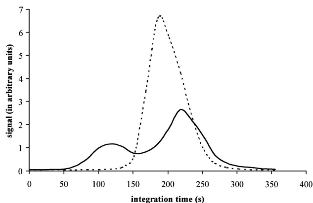
Fig. 6. Thermal profile of lignite-derived humic acid (dotted line) and of fine mode aerosol (solid line) from rural Hungary. From Gelecsner et al. (2000a; with permission).
