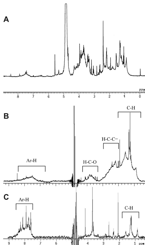
Fig. 3. (a) ^1\text{H} -NMR spectrum for HULIS extracted from NIST urban dust. From Havers et al. (1998; with permission); (b) ^1\text{H} -NMR spectrum for polyacidic fraction of an aerosol sample collected from the Po Valley. From Decasari et al. (2002; with permission); (c) ^1\text{H} -NMR spectrum for polyacidic fraction of \text{D}_2\text{O} extract of ozonised soot. From Decasari et al. (2002; with permission).
