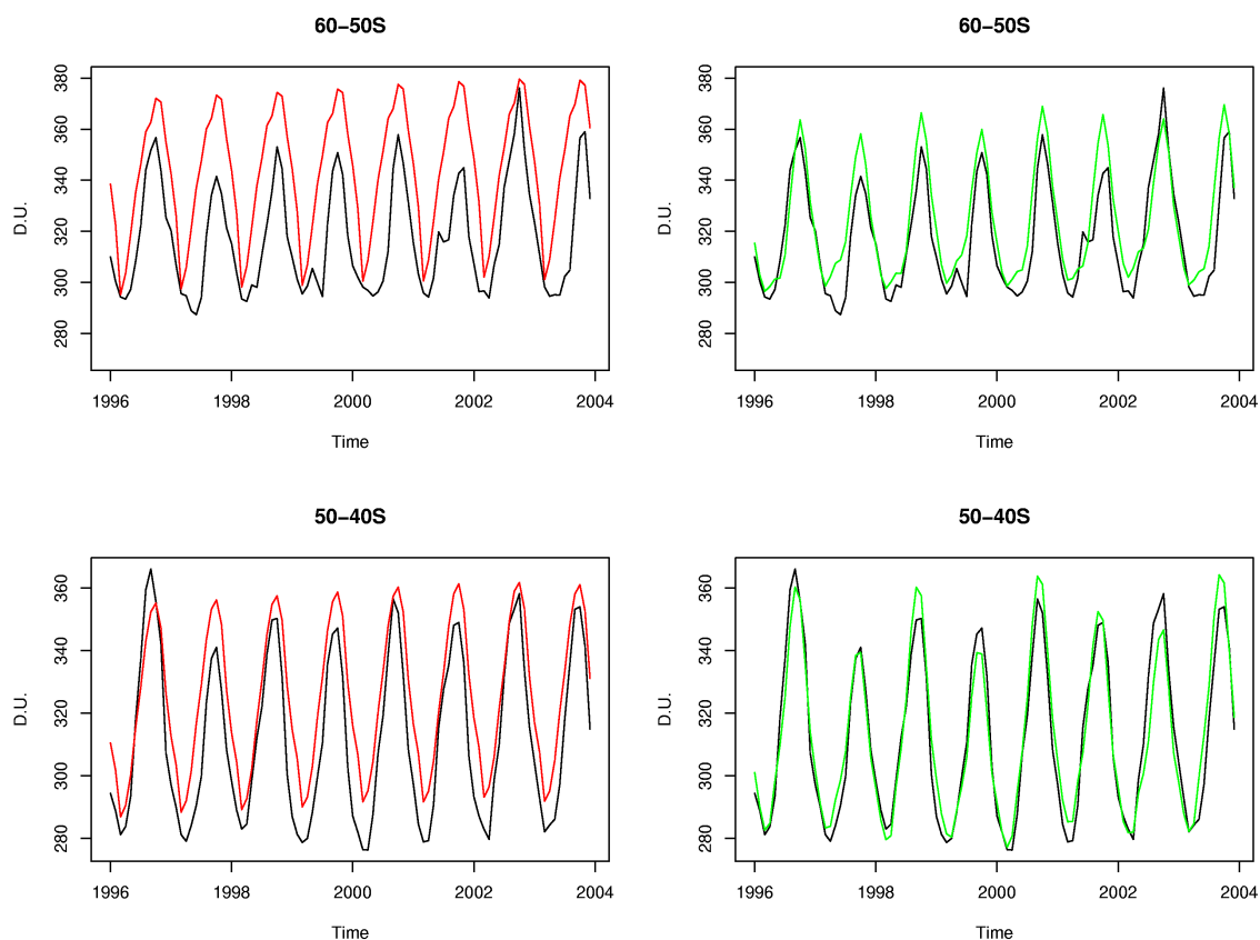
Fig. 4. Time series of measurements (black), UIUC 2-D model outputs (red), and statistically adjusted UIUC 2-D model outputs (green). In Dobson Units, 1996–2003, for latitude bands 60^{\circ} – 50^{\circ} S and 40^{\circ} – 50^{\circ} S.
