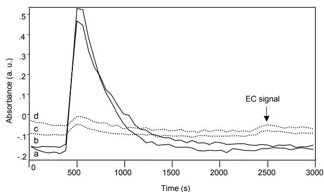
Fig. 5. CECs obtained by TGA/FT-IR analyzing a 24-hour sample of particulate matter (on a filter). The filter was divided into two portions both heated at 425°C for 25 min (curves a and b); curve c was obtained with the heating program, reported in Fig. 3, on one half of the filter submitted to 24-h Soxhlet extraction; curve d was obtained by the same heating program on the second half of the filter not extracted.
