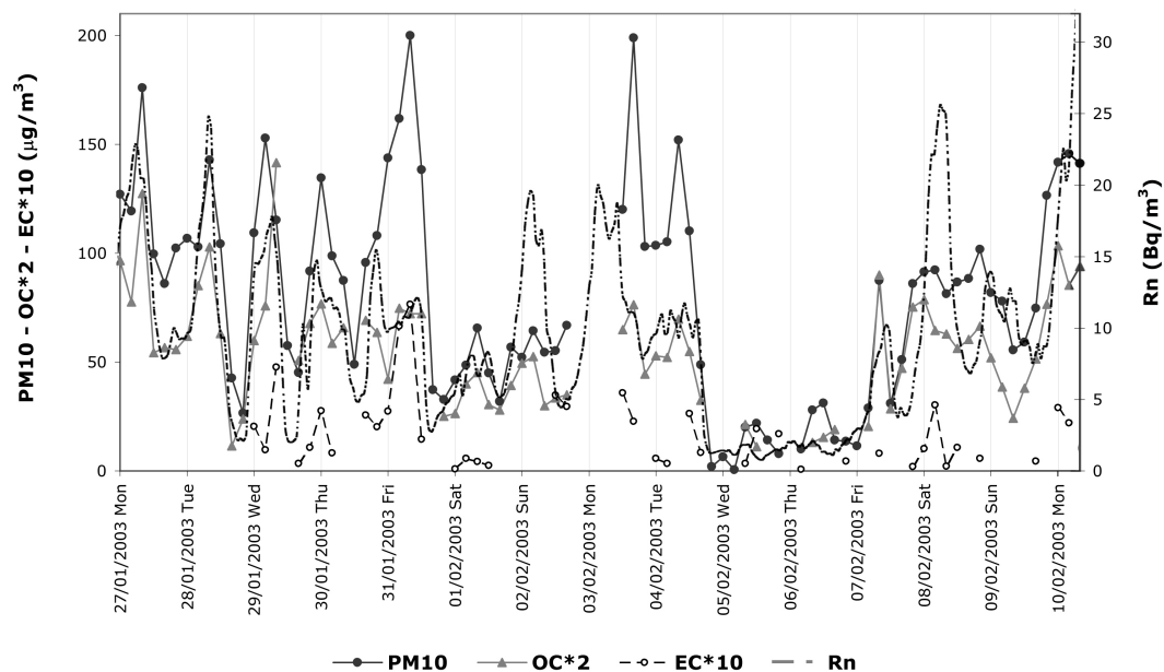
Fig. 10. Temporal patterns of PM10, OC and EC concentrations together with Radon concentration (OC and EC values have been multiplied x2 and x10 respectively).
