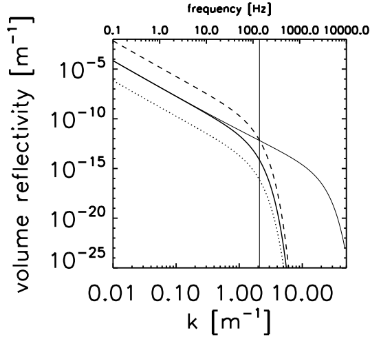
Fig. 6. Volume reflectivity as a function of wave number for various cases of electron densities N_e , Schmidt number Sc , and N_\vartheta . Standard case (thick solid curve): N_e=1\cdot 10^{10}/\text{m}^3 , N_\vartheta=1\cdot 10^{-5}/\text{s} , and Sc=1 . Relative to the standard case the electron density has been decreased by a factor of 10 (dotted line), N_\vartheta has been increased by a factor of 100 (dashed line), and the Schmidt number has been increased by a factor of 100 (thin solid line). The energy dissipation rate is \epsilon=0.1 W/kg and the kinematic viscosity is \nu=0.245 m 2 /s for all curves. The value for \nu is representative for an altitude of 70 km. The thin vertical line corresponds to the Bragg scale of the ALWIN radar.
