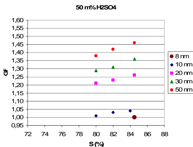
Fig. 7. Experimental growth factors (GFs) of ultrafine (8, 10, 20, 30 and 50 nm, respectively) particles with sulfuric acid mass fraction of 50% as a function of ethanol saturation ratio (S%). Error limits are inside the data points in the figure.
