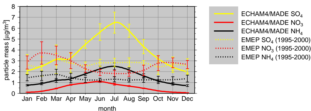
Fig. 7. Climatological seasonal cycle of observed and modeled near surface mass concentrations of the aerosol components \text{SO}_4 , \text{NO}_3 , and \text{NH}_4 in fine particles ( \text{PM}_{2.5} ), averaged over Europe. The error bars denote the standard deviation of the individual monthly means to the climatological average.
