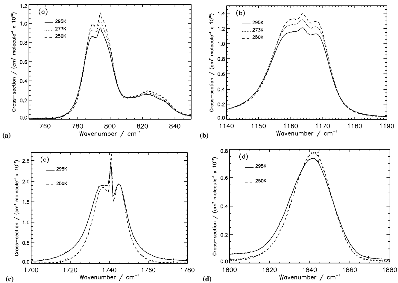
Fig. 2. A close up of the: (a) 794 , (b) 1163 , (c) 1741 and (d) 1842 \text{ cm}^{-1} PAN bands showing temperature dependence at 295 \text{ K} (solid line) 273 \text{ K} (dotted line) and 250 \text{ K} (dashed line). Note: 295 \text{ K} data taken from Allen et al. (2005).
