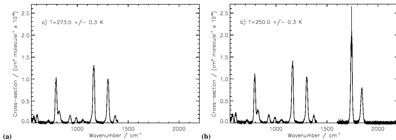
Fig. 1. PAN mid-infrared absorption cross-sections ( 0.25 \text{ cm}^{-1} resolution) at sample temperatures of: (a) 273 \text{ K} \pm 0.3 \text{ K} ( 550 – 1400 \text{ cm}^{-1} ); and (b) 250 \pm 0.3 \text{ K} ( 550 – 1400 \text{ cm}^{-1} , 1600 – 2000 \text{ cm}^{-1} ). Note: measurements at 273 \text{ K} were not made above 1600 \text{ cm}^{-1}
