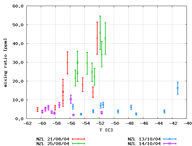
Fig. 1. H 2 O-mixing ratio plotted versus ambient temperature. The samples can clearly be separated into stratospheric samples with \nu < 10 ppm, and samples from the tropopause region, which still show a temperature dependence.
