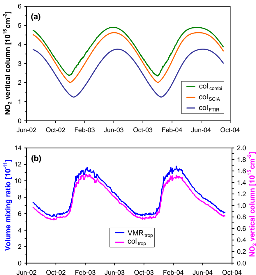
Fig. 11. (a) Total column series col_{combi} (green) inferred from the combined a-posteriori retrieval from FTIR and SCIAMACHY data. Column series retrieved from SCIAMACHY alone col_{SCIA} (orange, same as in Fig. 5) and the column series retrieved from FTIR alone col_{FTIR} (blue, same as in Fig. 5). (b) Time series of the clean background tropospheric mixing ratio VMR_{trop} obtained from the combined retrieval of FTIR and SCIAMACHY (blue), and the corresponding clean background tropospheric column between 1.077 km–10 km ( col_{trop} , magenta).
