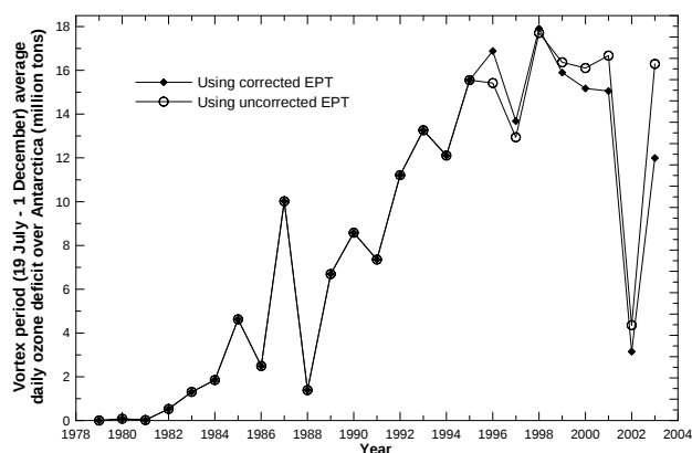
Fig. 15. The AVP mean ozone mass deficit ( \text{O}_3 < 220 DU) for each year in 10^9 kg. Values derived using the EPT data corrected after comparison with Dobson spectrophotometer measurements are shown using diamonds, while values derived using uncorrected EPT data are shown using circles.
