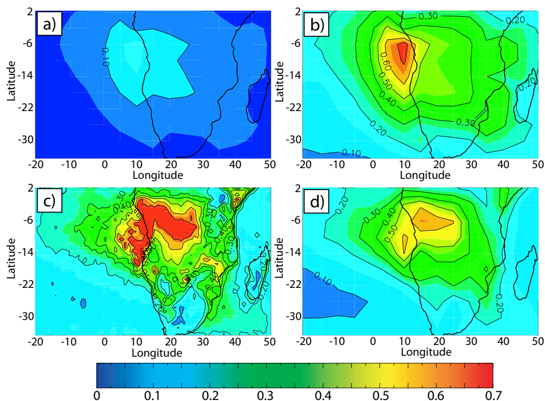
Fig. 3. Monthly mean aerosol optical depth for September at a wavelength of 0.55 \mu\text{m} for (a) OC+BC component in the GCM; (b) OC+BC component in GCM increased by a factor of 4.4 as derived from comparison with AERONET measurements; (c) MODIS total column (2000–2003 average); (d) MODIS data aggregated to the GCM resolution and \times 0.84 to estimate the biomass burning aerosol fraction. The MODIS data is linearly interpolated to missing data regions over arid land areas where the surface reflectance exceeds the threshold value required for the aerosol retrieval.
