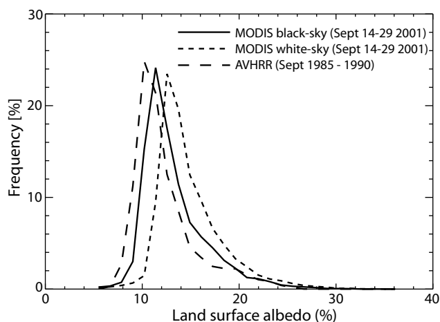
Fig. 8. Histograms of land surface albedo at 0.25° resolution for southern Africa for the MODIS black and white-sky (0.3–5.0 \mu\text{m} ), and AVHRR (0.35–3.0 \mu\text{m} ) albedo retrievals. The bin size in the histogram is 1.2%.
