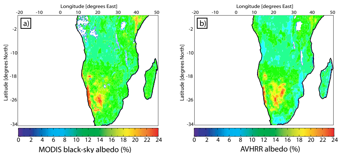
Fig. 7. (a) MODIS black-sky albedo (0.3–5.0 \mu\text{m} ) at 0.25° resolution for the period 14–29 September 2001 and (b) AVHRR albedo (0.35–3.0 \mu\text{m} ) at 0.25° resolution for September averaged over a five year period (1985–1987, 1989–1990). White pixels over land regions in the MODIS data set represents missing data values.
