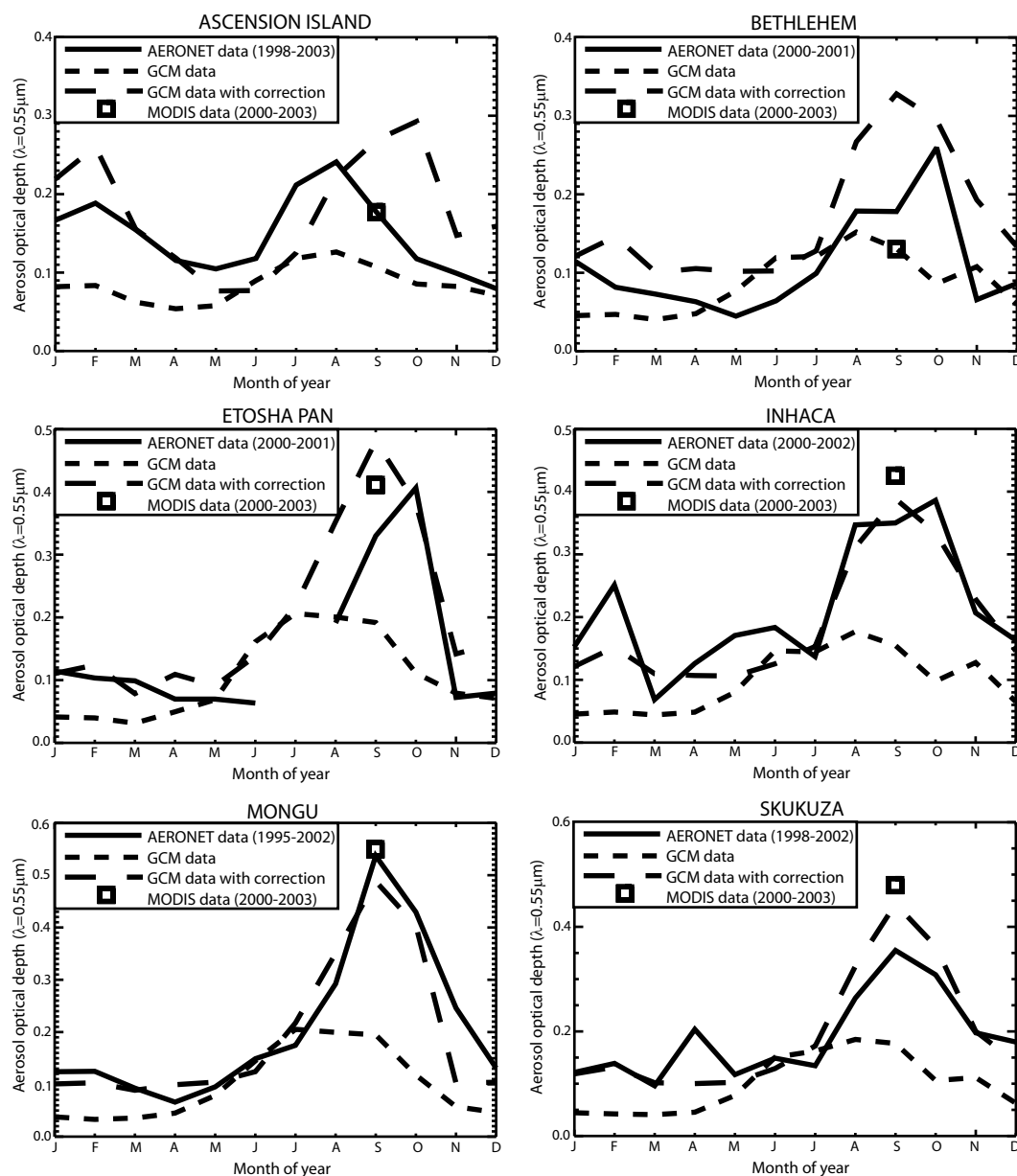
Fig. 2. Comparison of the monthly mean column integrated aerosol optical depth at 0.55 μm from the GCM of Tegen et al. (1997) with values measured at 6 AERONET sites. The years where the AERONET data was obtained is indicated on the individual plots. Also shown is the monthly mean value with a correction factor applied to the GCM data derived from a linear fit to the AERONET measurements (see Table 1), and the mean MODIS aerosol optical depth ( 1 \times 1^\circ ) for September (2000–2003 average) co-incident with the AERONET site.
