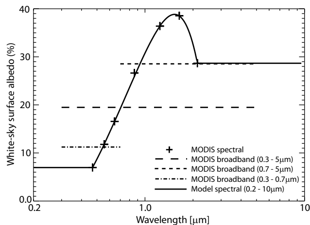
Fig. 9. MODIS white-sky albedo as a function of wavelength for 14–29 September 2001 aggregated to the model resolution ( 4 \times 5^{\circ} ) for the grid box centred at -22^{\circ} N, 20^{\circ} E. Shown are the three broadband retrievals at 0.3\text{--}0.7 \mu\text{m} , 0.7\text{--}5 \mu\text{m} , 0.3\text{--}5 \mu\text{m} , and the spectral dependent albedo derived from seven of the MODIS wavebands. Also indicated is the spectral albedo included in the model using least squares fitting with a quadratic of the form y=a+bx+cx^2 to the spectral measurements at \lambda=0.47\text{--}2.13 \mu\text{m} , and extrapolated at a constant value for wavelengths outside of this range.
