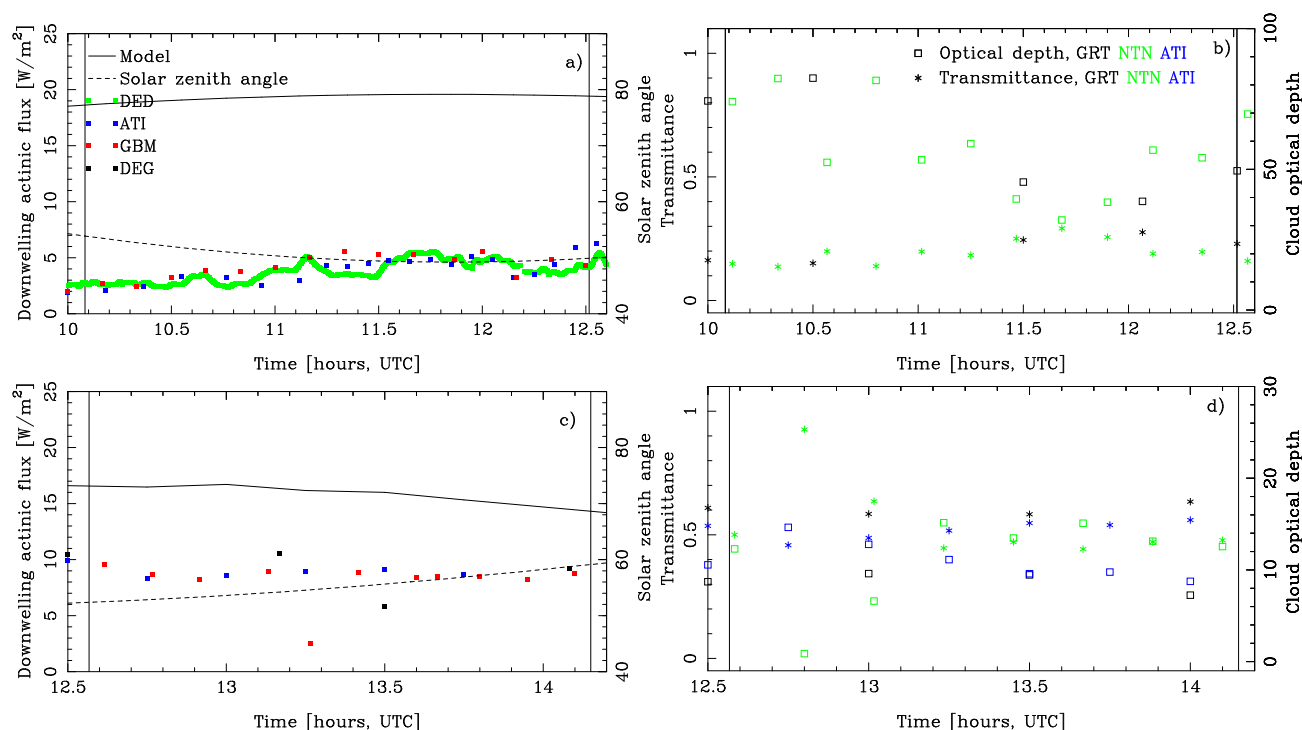
Fig. 3. Downwelling actinic fluxes integrated between 380–400 nm at the ground, (a) day 257 and (c) day 263, as measured in Weybourne (ATI, blue points), Beeston (GBM, red points), Briston (DEG, black points) and Aylsham (DED, green points). No data are available from the DED instrument on day 263. The black solid lines are cloudless model results for Weybourne, and the black dashed line is the solar zenith angle. In (b) and (d) are shown the effective cloud optical depths (squares) and the cloud transmittances (asterisks) for day 257, (b), and 263, (d). The black colours represent data from the GRT instrument, green the NTN instrument, and blue the ATI instrument. The black vertical lines indicate the interval in which the flights took place. Note different scales on y-axes of optical depth.
