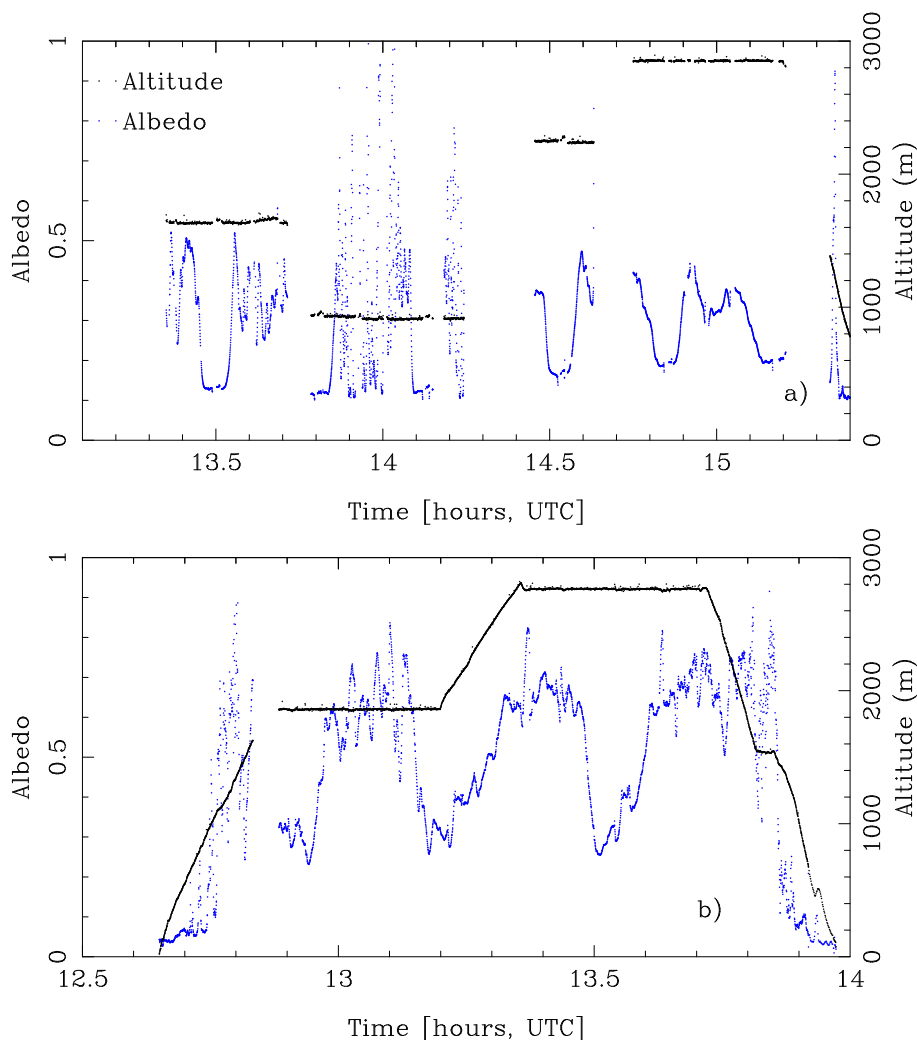
Fig. 14. Albedo at 380 nm measured during the flights on day 256, (a), and day 261, (b). The albedo is derived from irradiance measurements onboard the Partenavia. The black solid lines show the altitude of the aircraft. Data points where the pitch of the aircraft was larger than 5^\circ or the roll was larger than 1^\circ have been excluded.
