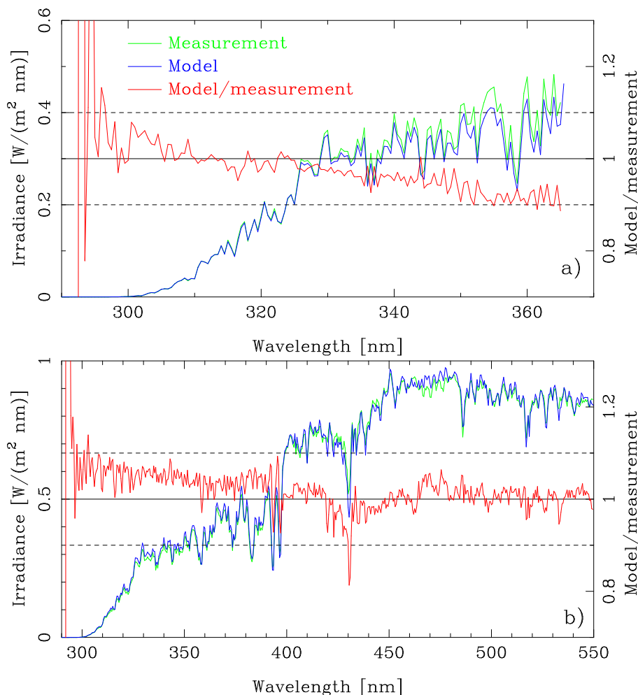
Fig. 1. Measured irradiance spectra, green lines, from the GRT instrument located at Bristol, (a) and the NTN instrument at Aylsham, (b). The spectra were recorded at 14:00 UTC on day 255. In blue is shown the uvspec model simulations of the spectra. The red lines are the model/measurement ratios. Note the different scales on the x-axes in a) and b).
