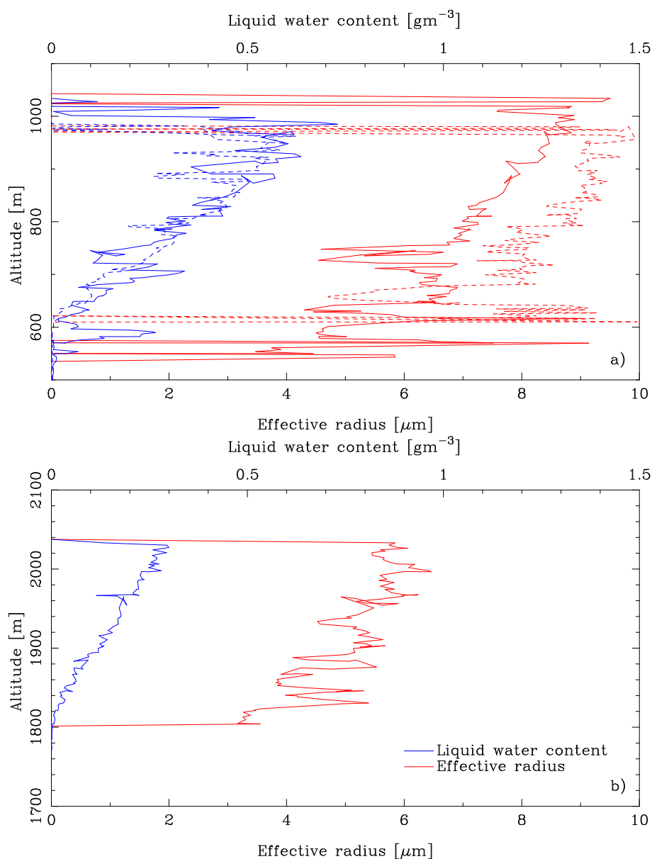
Fig. 2. Liquid water content (blue lines) as measured by the PVM instrument and the effective radius (red lines) measured by the Fast-FSSP instrument. In (a) the solid lines are from the descent and the dashed lines from the subsequent ascent on day 257. In (b) the data are from day 263. Note different scales on the y-axes.
