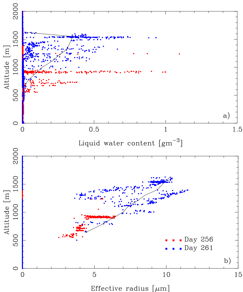
Fig. 15. Liquid water content, (a), as measured by the PVM instrument and the effective radius, (b), measured by the Fast-FSSP instrument. Red dots are data from day 256 and blue dots data from day 261. The solid lines are the input used for the model simulations.
