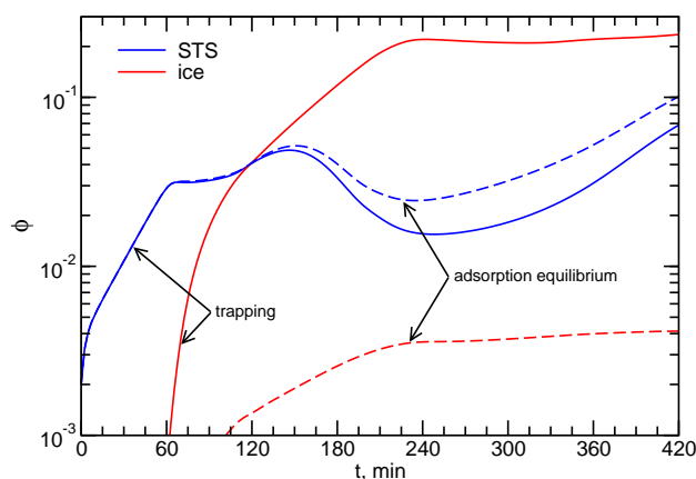
Fig. 9. As Fig. 8, again with the solid curves representing the baseline case but now on a logarithmic scale. The dashed curves have been obtained by assuming instantaneous adsorption equilibrium of \text{HNO}_3 on ice according to a saturated dissociative Langmuir isotherm, as frequently done in the interpretation of uptake data.
