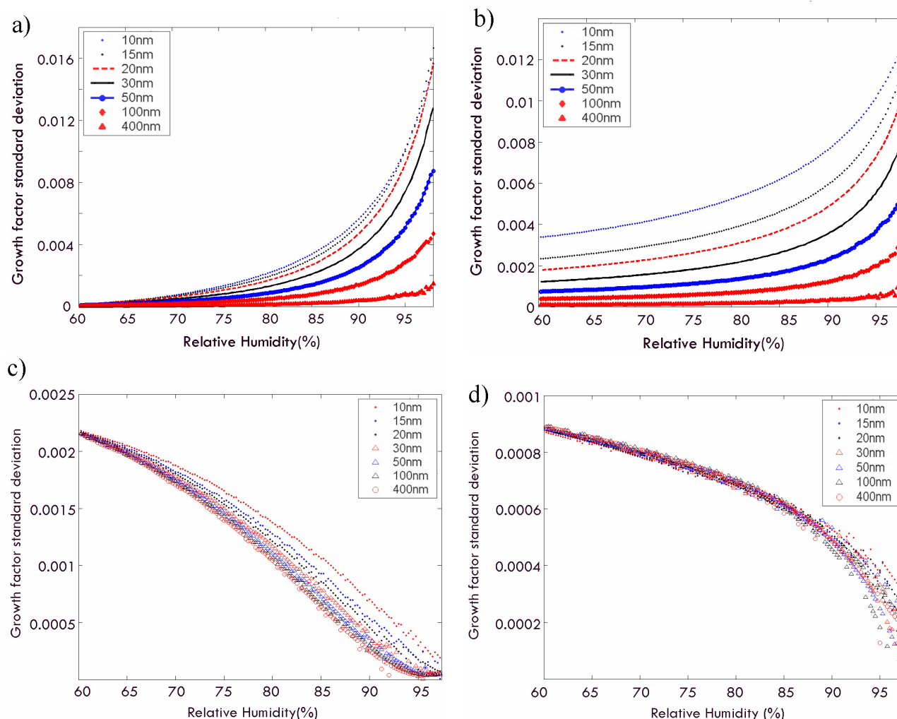
Fig. 8. (a) GF standard deviation for different dry diameters using 3 surface tension models for equimolar NaCl-(NH 4 ) 2 SO 4 at 25°C. (b) GF standard deviation for different dry diameters using 3 surface tension models for H 2 SO 4 -(NH 4 ) 2 SO 4 particles at 25°C. (c) GF standard deviation for different dry diameters using 3 solution density models for equimolar NaCl-(NH 4 ) 2 SO 4 particles at 25°C. (d) GF standard deviation for different dry diameters using 3 solution density models for equimolar H 2 SO 4 -(NH 4 ) 2 SO 4 particles at 25°C.
