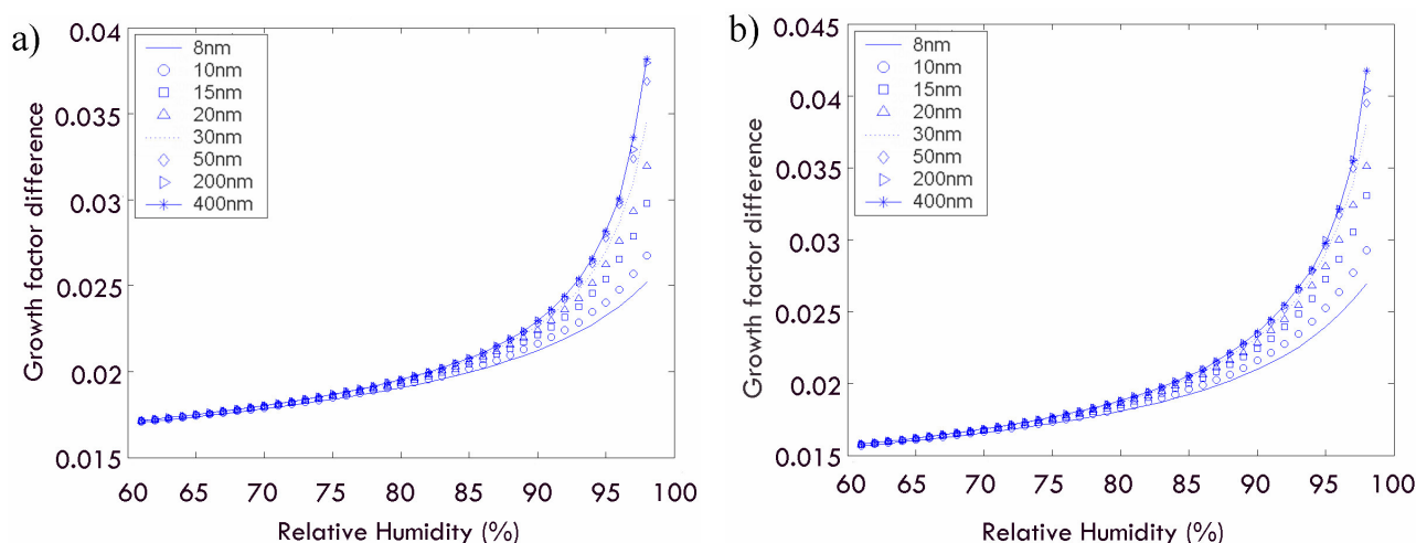
Fig. 9. (a) Growth factor difference for a (\text{NH}_4)_2\text{SO}_4 particle at 25°C and various dry diameters using two different density values. Values used were 1.769 \text{ kg/m}^3 (Perry's Chemical handbook) and 1.7 \text{ kg/m}^3 (Hameri et al., 2000). (b) Growth factor difference for a \text{NH}_4\text{NO}_3 particle at 25°C and various dry diameters using two different density values of 1.725 \text{ kg/m}^3 (rhombic crystal) and 1.66 \text{ kg/m}^3 (tetragonal crystal). Both values taken from Perry's Chemical handbook.
