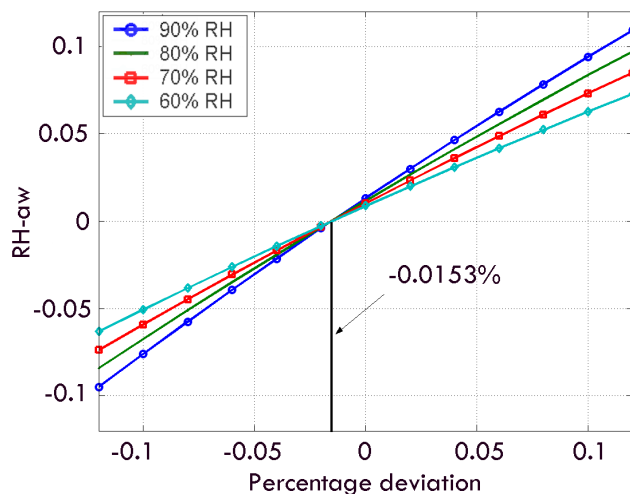
Fig. 7. Difference between equilibrium solution water activity and RH (0–1) for various values of \Delta G_f^\circ \text{H}_2\text{O(l)} . Percentage deviation is taken from the tabulated value of Ansari and Pandis (1999).
