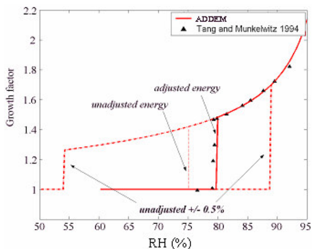
Fig. 6. Deliquescence growth curve for (\text{NH}_4)_2\text{SO}_4 – Sensitivity to Gibbs energy of formation for the salt.
