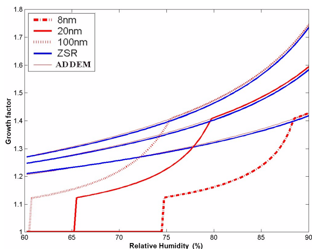
Fig. 4. Influence of curvature on aerosol composition for a mixed equimolar (\text{NH}_4)_2\text{SO}_4 - \text{NH}_4\text{NO}_3 aerosol at 25^\circ\text{C} . The model output (ADDEM) is from the scheme described in this paper including diameter dependence. The three dry diameters chosen are 8, 20 and 100 nm. Also shown are the growth factor predictions for a ZSR analogue growth factor model. Both utilise the mass fraction mixing rule of Tang (1997) for calculating the solution and dry densities.
