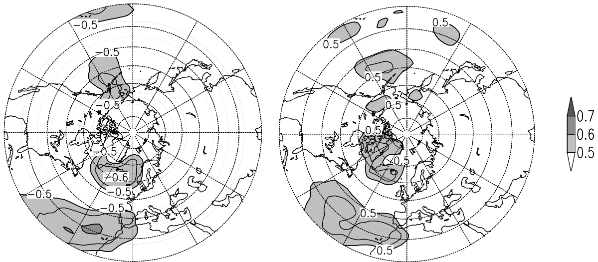
Fig. 2. As in Fig. 1, but for 15-day low pass filtered data at the 1000 hPa level. The isoline interval is 0.05. Only values larger than 0.5 are shown.
