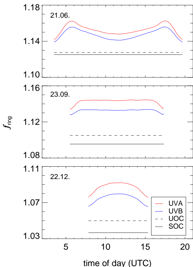
Fig. 12. Numerical ring correction factors f_{\text{ring}} on three days of the year. UV-A, UV-B: clear sky radiance distributions according to Grant et al. (1997). SOC, UOC: overcast radiance distributions. Plot ranges indicates times where \vartheta_{\circ} \leq 90^{\circ} .
