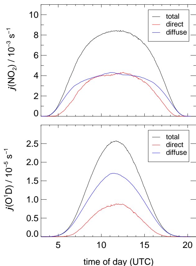
Fig. 14. Diurnal variations of j(\text{NO}_2) (upper panel) and j(\text{O}^1\text{D}) (lower panel) under clear sky conditions (28 July 2002). The contributions of direct and diffuse radiation show slight variations which are compensating each other. Such variations are very common on clear sky days and can be attributed to changes in aerosol load.
