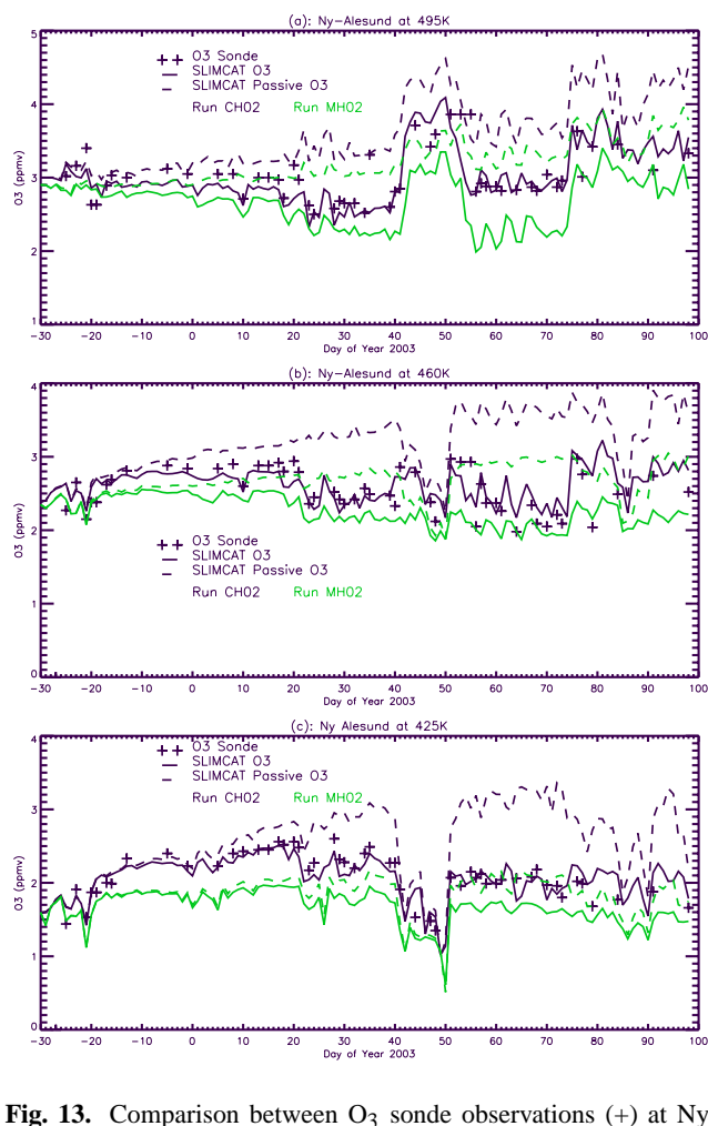
Fig. 13. Comparison between O 3 sonde observations (+) at Ny-Ålesund and results from the 2.8^\circ \times 2.8^\circ resolution SLIMCAT runs CH02 (CCM, high resolution) and MH02 (MIDRAD, high resolution) for winter 2002/2003 (top: 495 K, middle: 460 K, bottom: 425 K).
