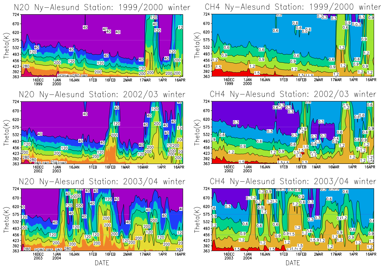
Fig. 2. Model \text{N}_2\text{O} (ppbv) and \text{CH}_4 (ppmv) at Ny-Ålesund station ( 79^\circ\text{N} , 12^\circ\text{E} ) from SLIMCAT runs CH99, CH02, and CH03 (CCM, high resolution) as a function of time and \theta for the three Arctic winters (top: 1999/2000, middle: 2002/2003, bottom: 2003/2004).
